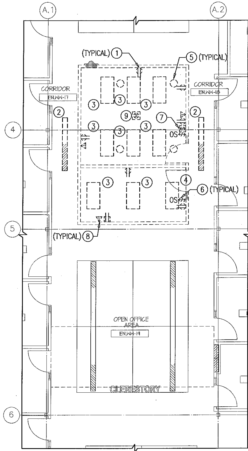
1 PART MAIN FLOOR DEMOLITION PLAN - ELECTRICAL E0.2 SCALE: 1:100
