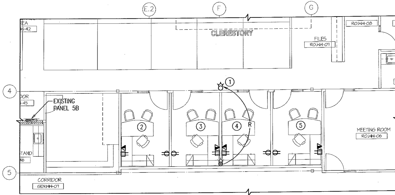
1 PART MAIN FLOOR PLAN - POWER & SYSTEMS SCALE: 1:100
