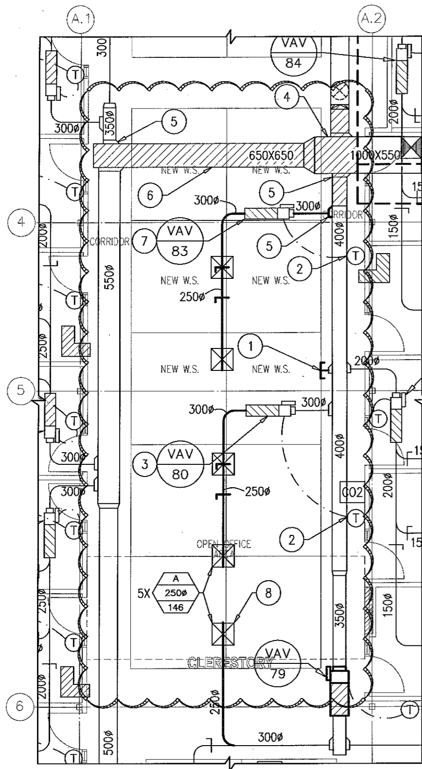
1 PART MAIN FLOOR PLAN - MECHANICAL M-2 SCALE: 1:100
