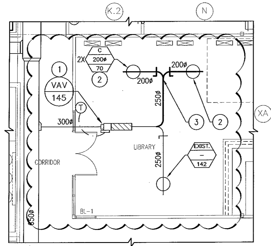
1 PART MAIN FLOOR PLAN - MECHANICAL M-3 SCALE: 1:100
