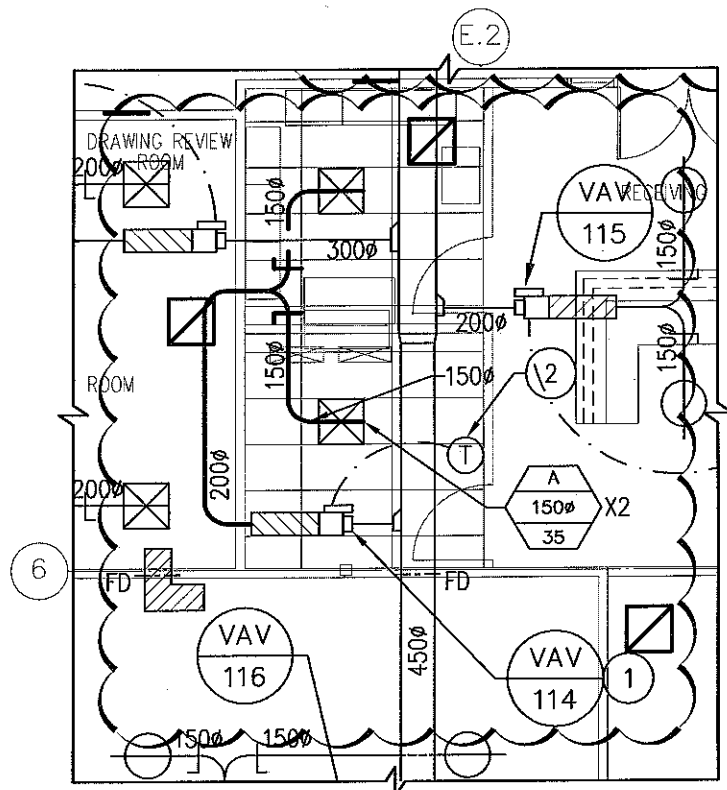
1 PART MAIN FLOOR PLAN - MECHANICAL M-4 SCALE: 1:100
