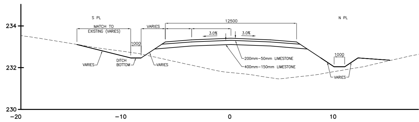
CROSS SECTION 1:100H; 1:50V
