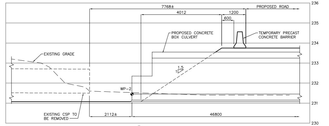
CROSS SECTION 1:50
