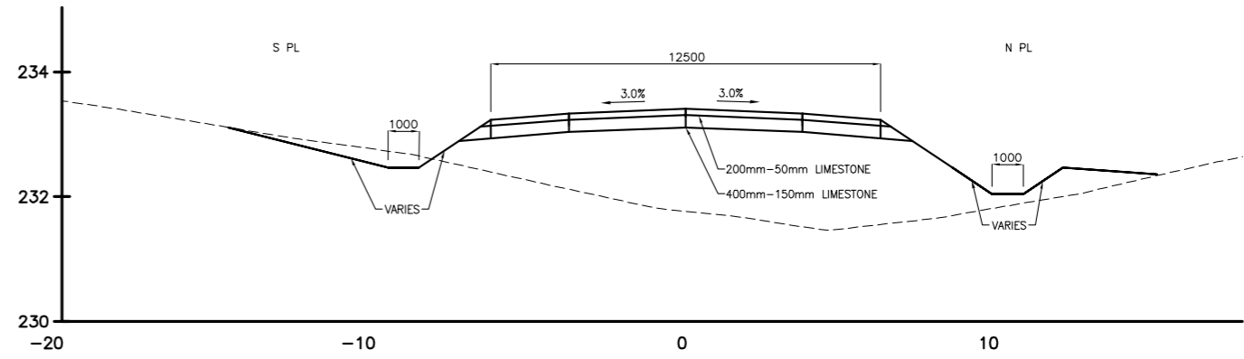
A 5 5 CROSS SECTION AT STA. 2+250 1:100H; 1:50V
