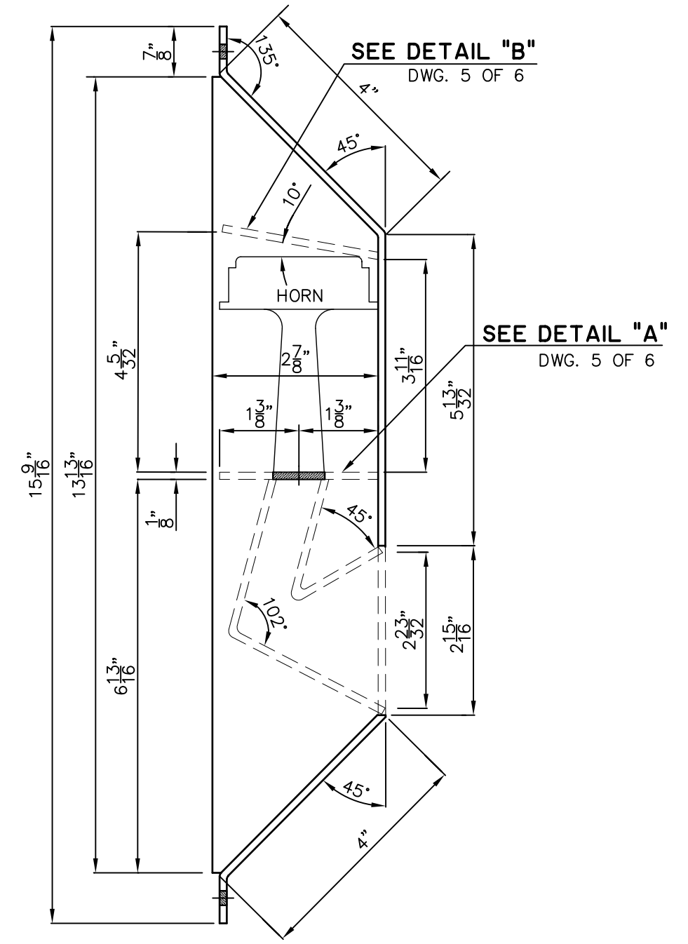
SIDE VIEW
