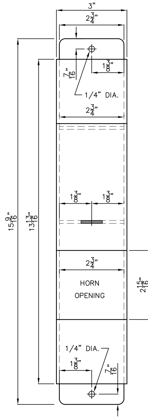
FRONT VIEW
