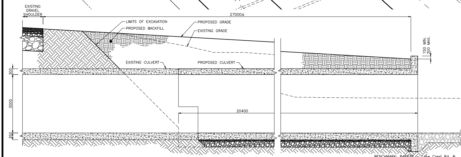
A SECTION 1:50
