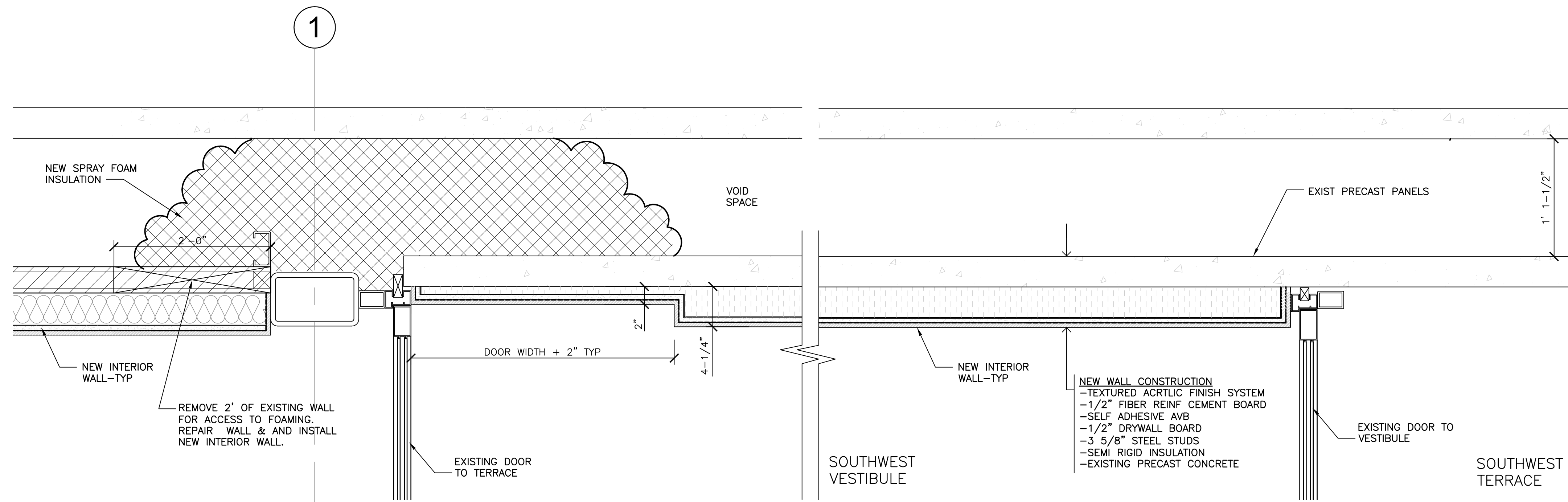
1 SW VESTIBULE INSULATION DETAIL SCALE: 1 1/2"=1'-0"
