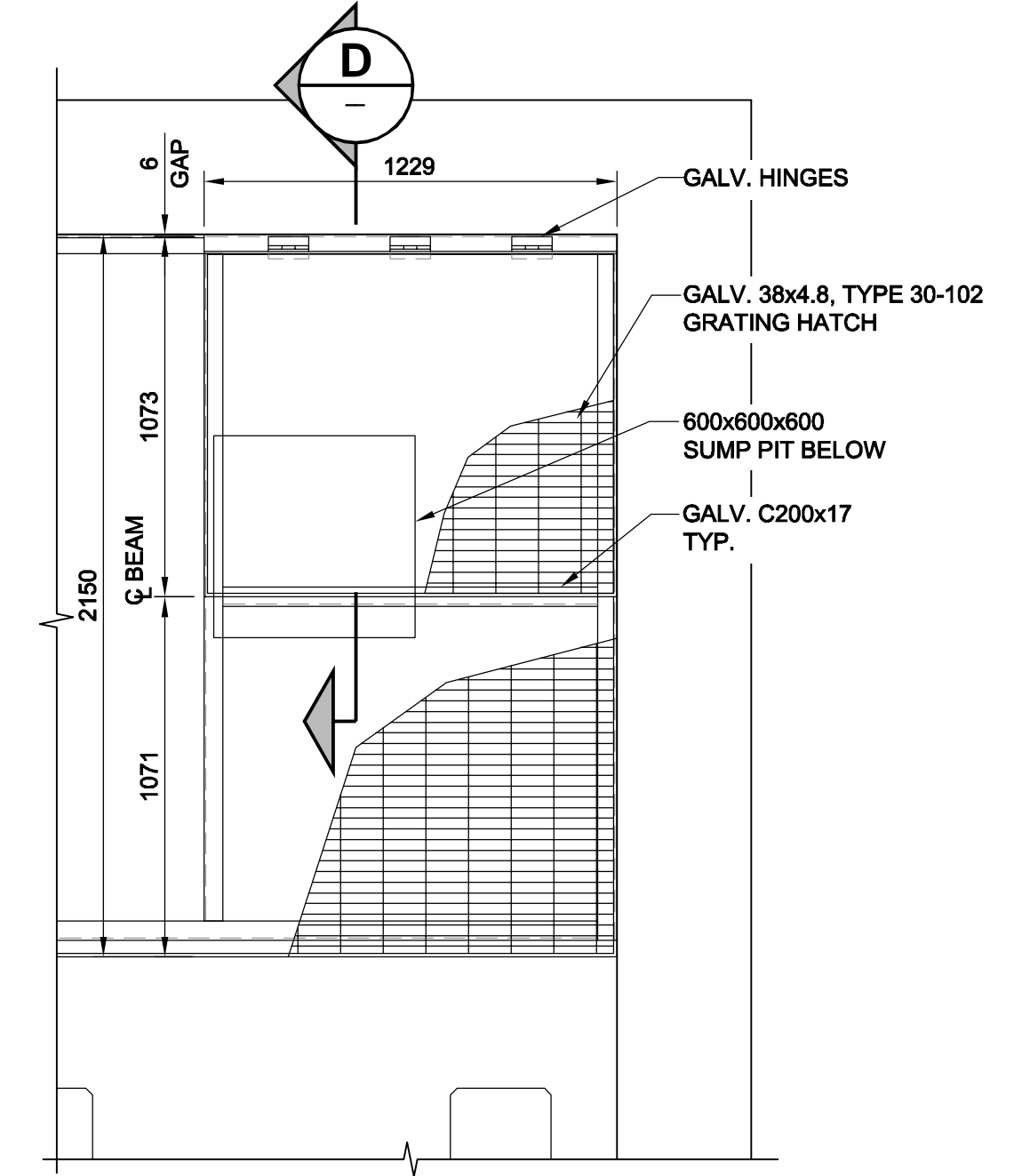
DETAIL 19 D-11923 SCALE 1:20
