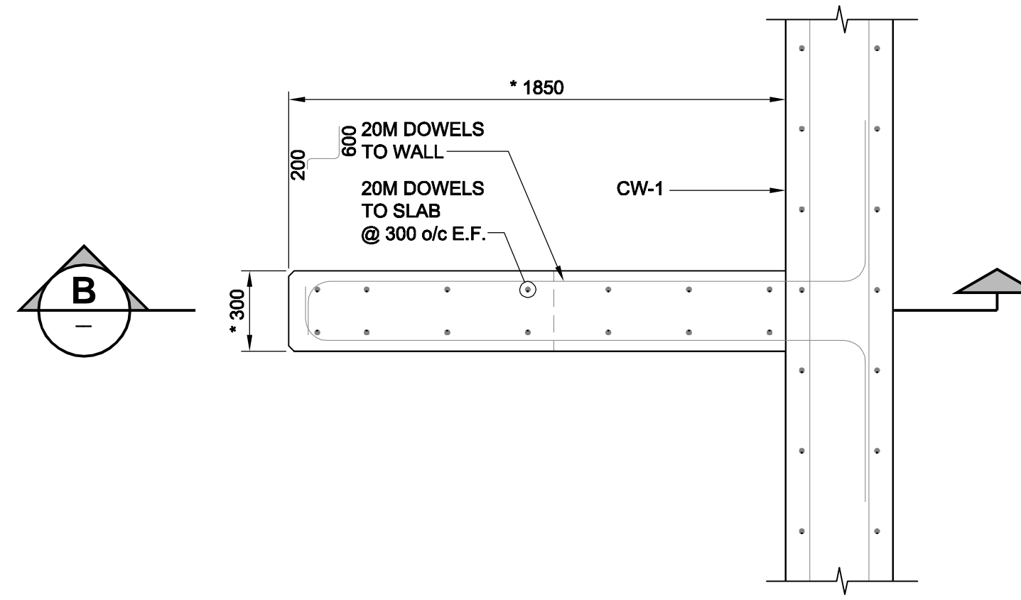
DETAIL 18 D-11923 SCALE 1:20
