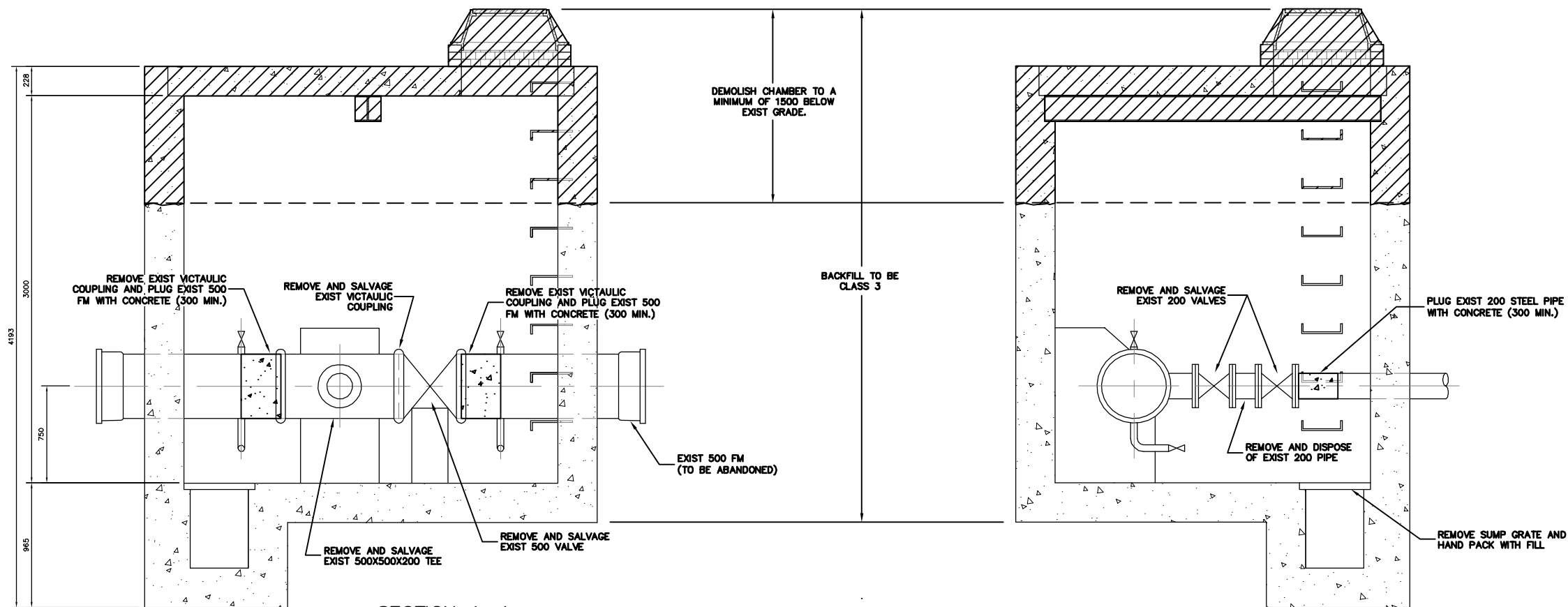
SECTION B-B SCALE 1:20
