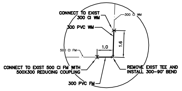
DETAIL "C" NTS
