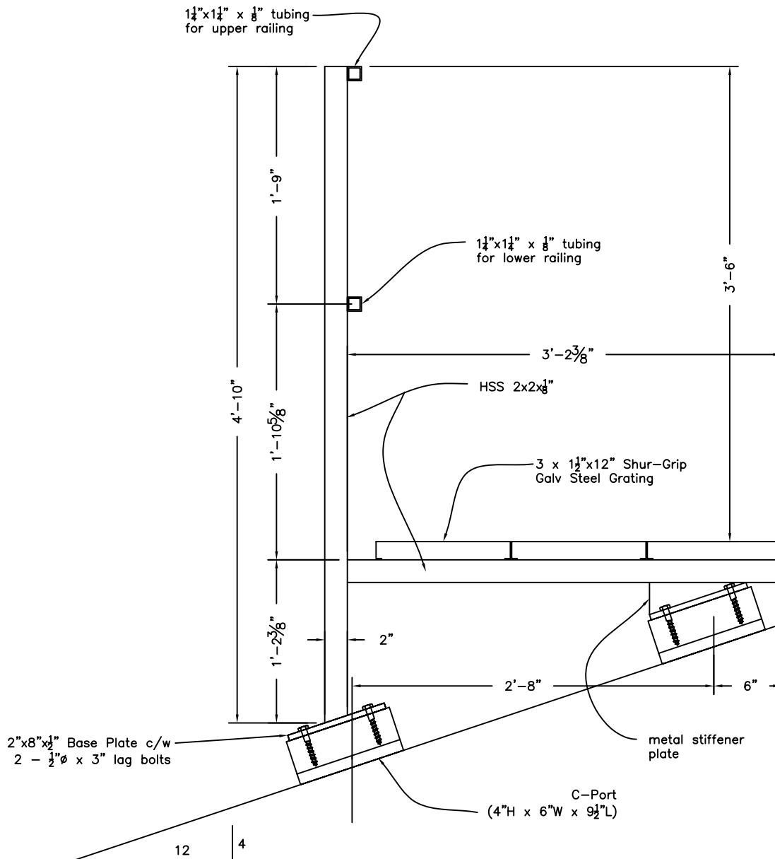
Side Detail 1" = 1'-0"
