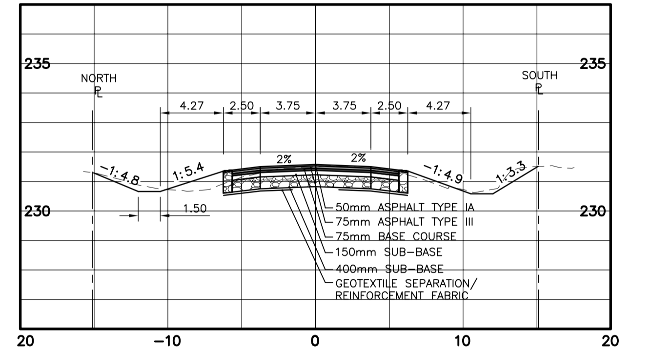
A SECTION AT STA 1+340 1:250H 1:125V
