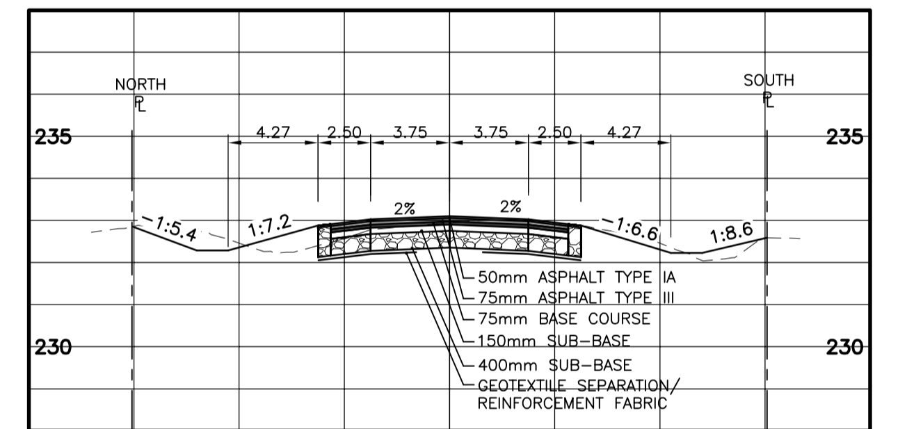
SECTION AT STA 1+850 1:250H 1:125V
