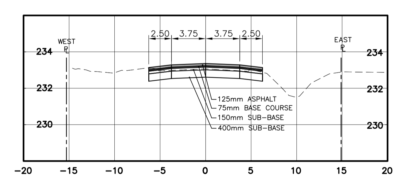
A SECTION AT STA 1+050 1:250H 1:125V
