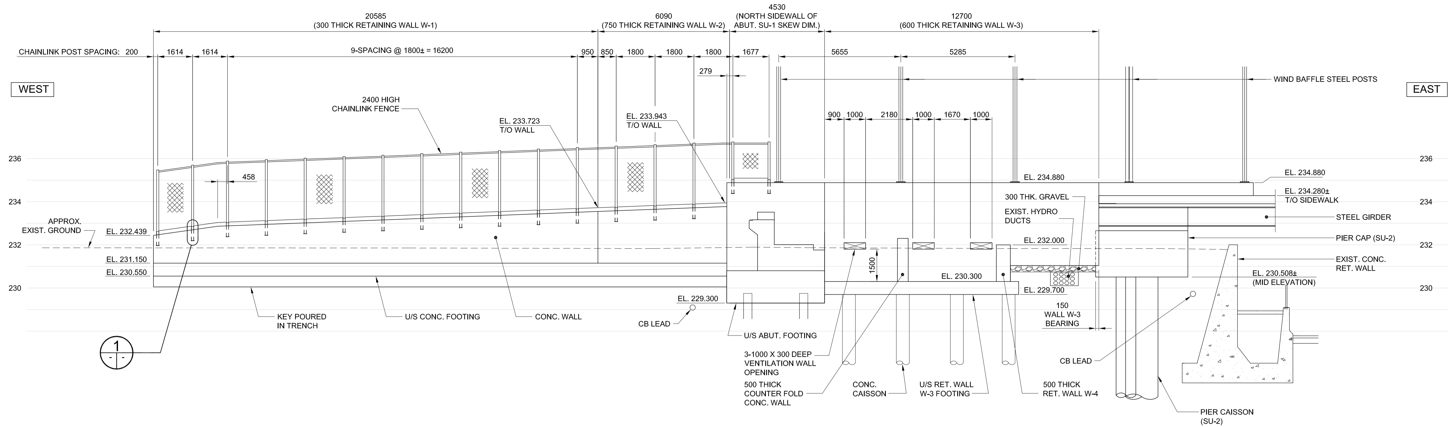
SECTION F SCALE 1:100
