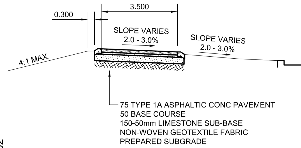
TYPICAL SECTION MULTI-USE PATH FRONTING LINDSAY STREET
