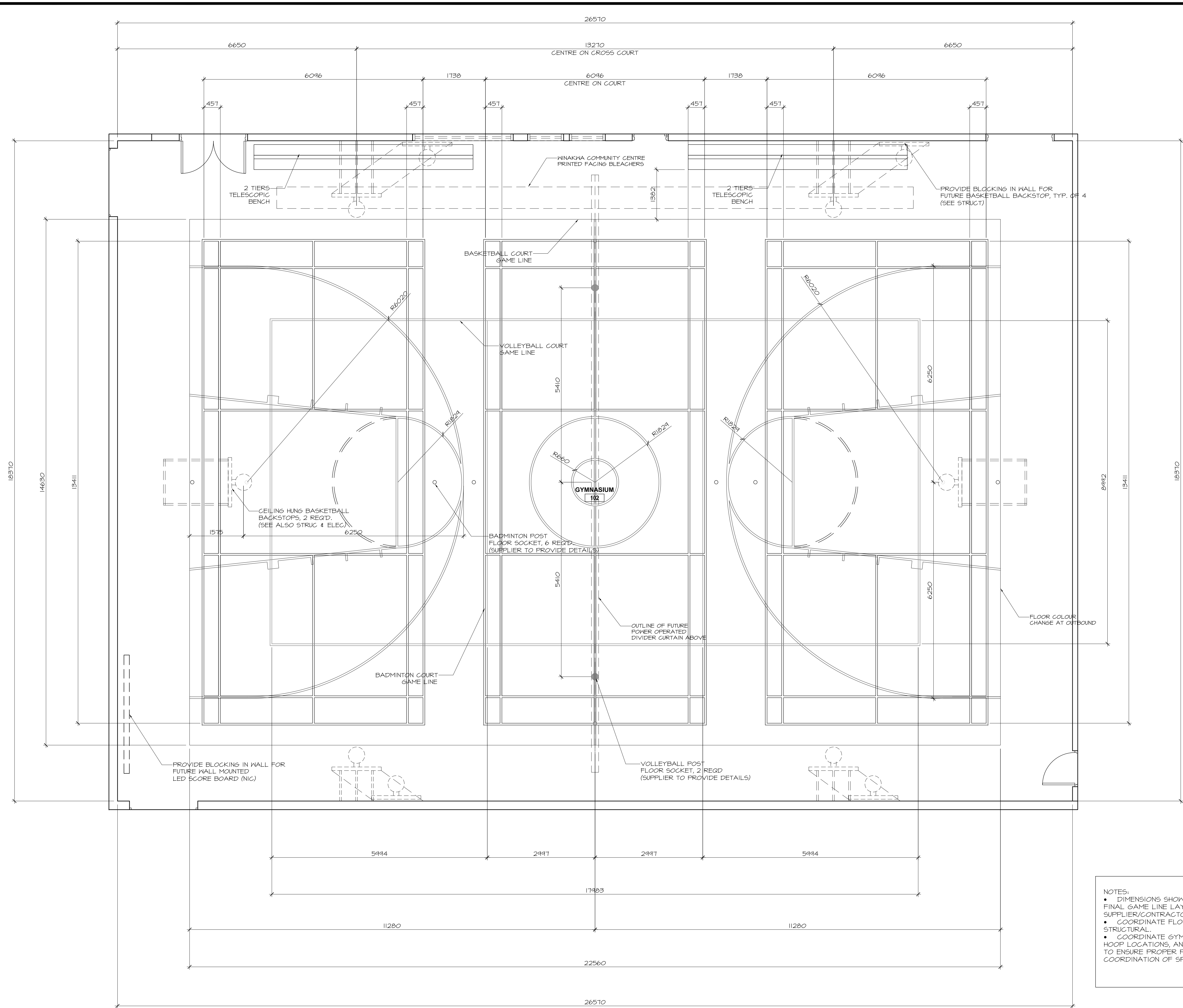
1 2.4 COURTS GAME LINE LAYOUT
