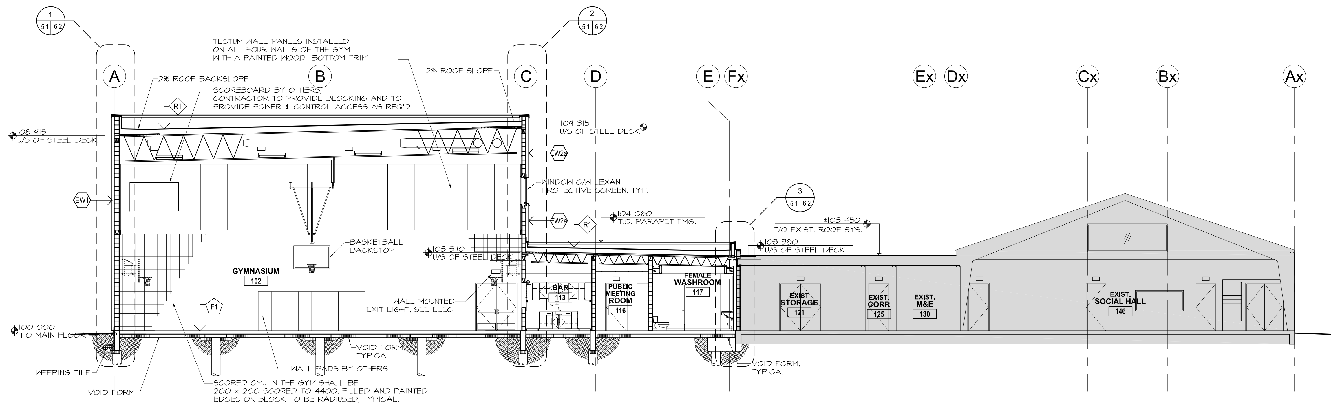
2 BUILDING SECTION 2.1 5.1 1:100
