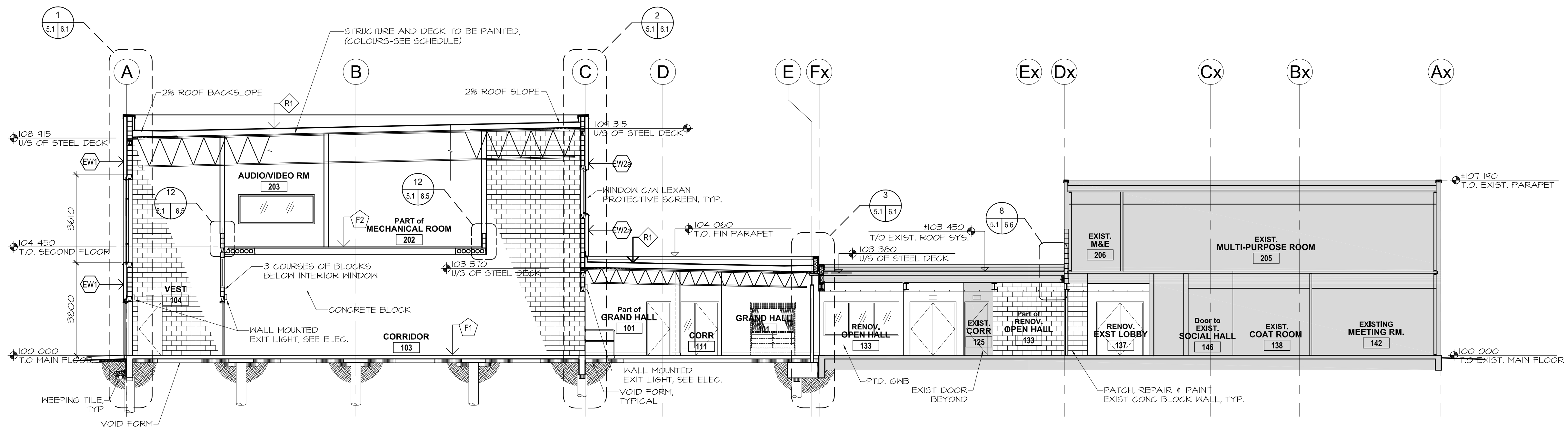
1 BUILDING SECTION 2.1 5.1 1:100
