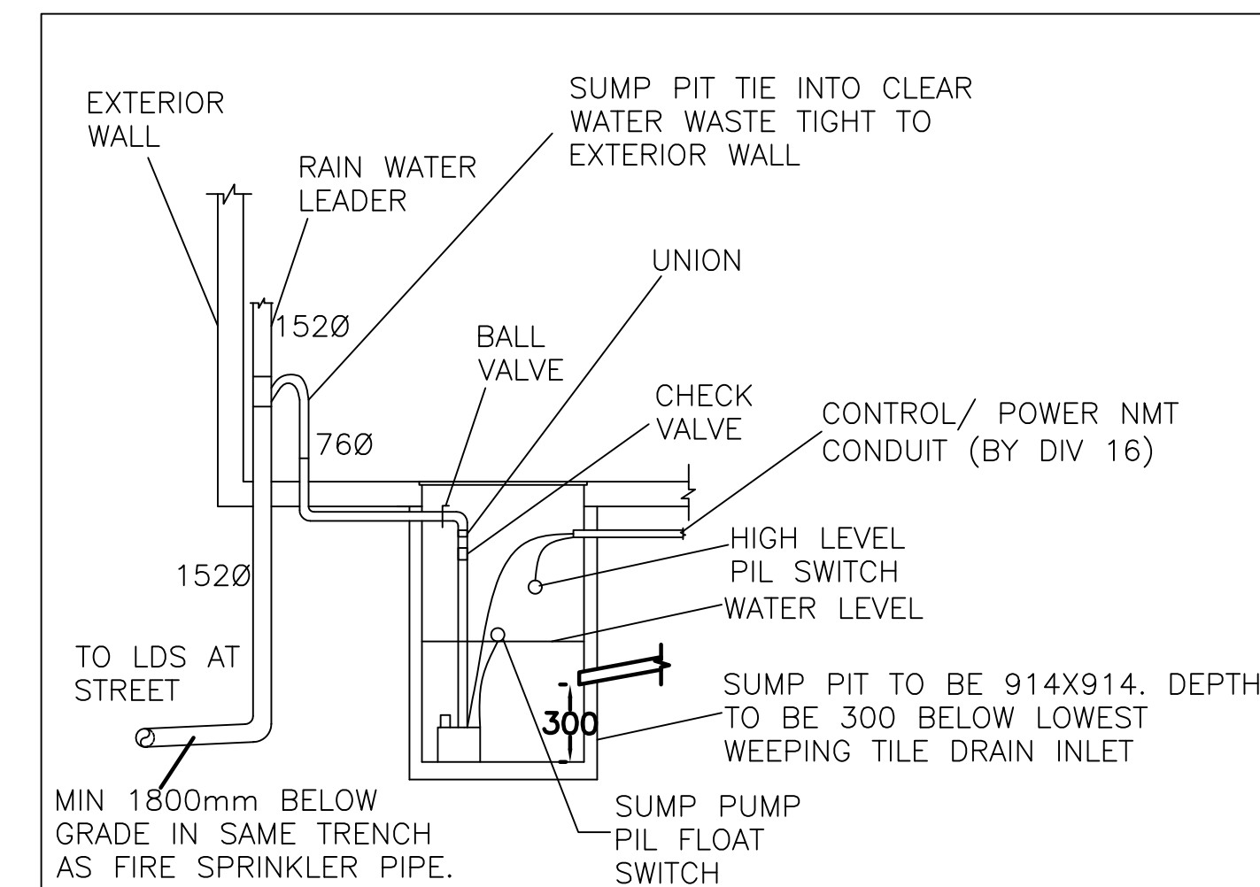
2 SUMP PUMP PIPING DETAIL M-3.1 SCALE: 1:100
