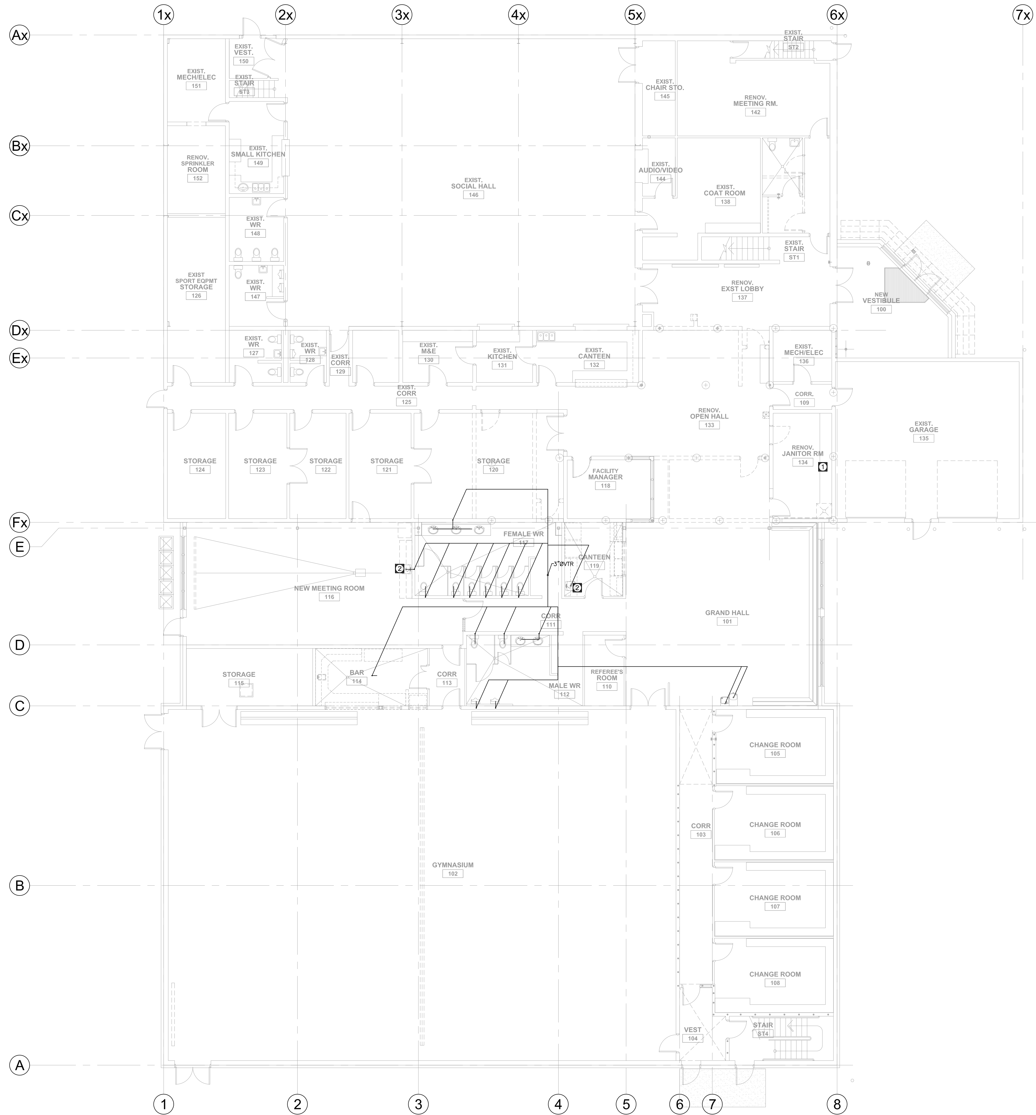
1 VENT PIPING SCHEMATIC MAIN FLOOR M-3.4 SCALE: 1:100
