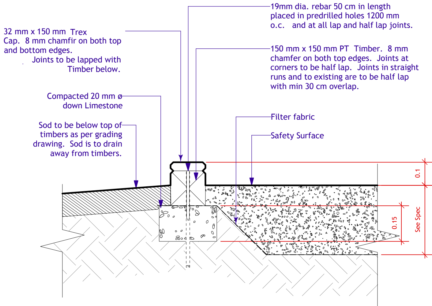
2 Timber Play Curb (1 Layer) w. Cap L-6 Scale: 1:10
