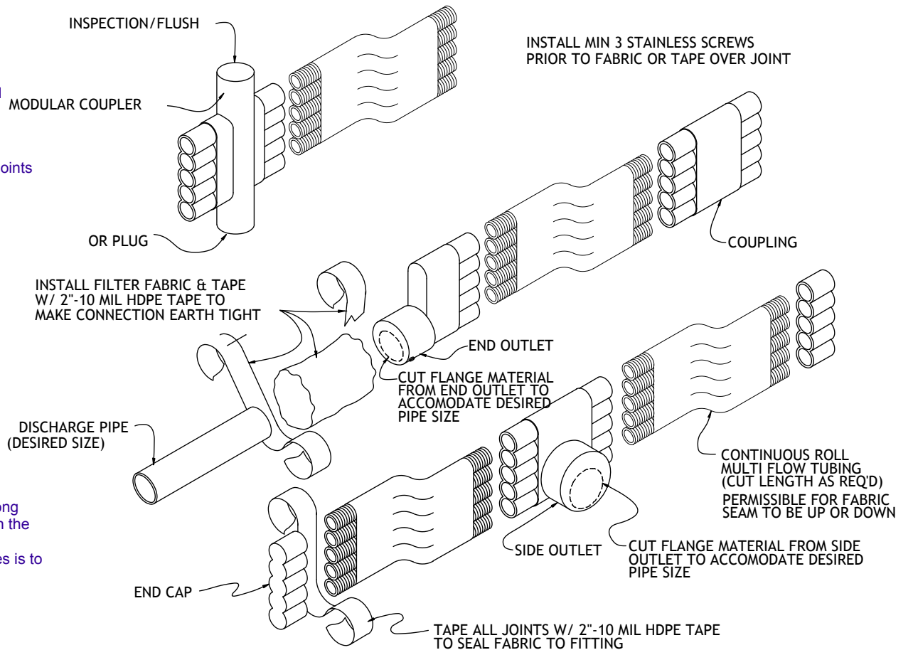
1 Multi Flo Connection Details L-7 Scale: 1:5
