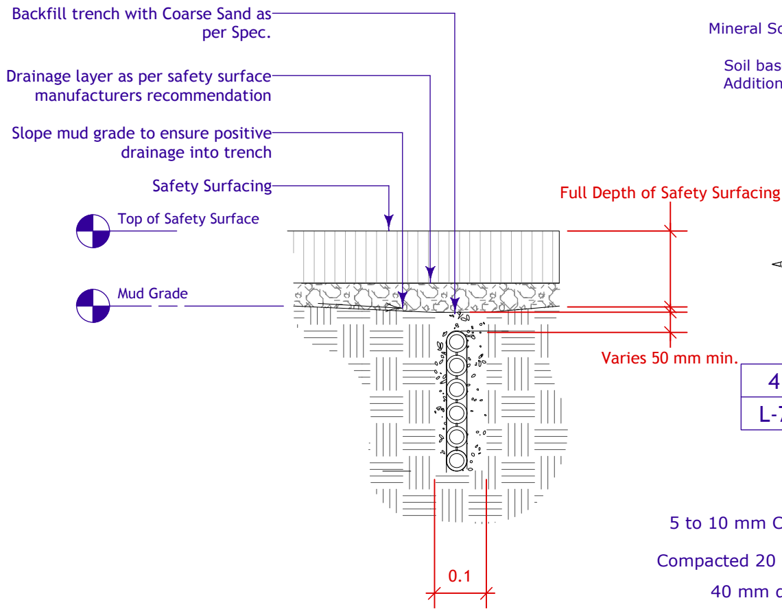
2 Multi Flo Trench under Play Safety Surface L-7 Scale: 1:10
