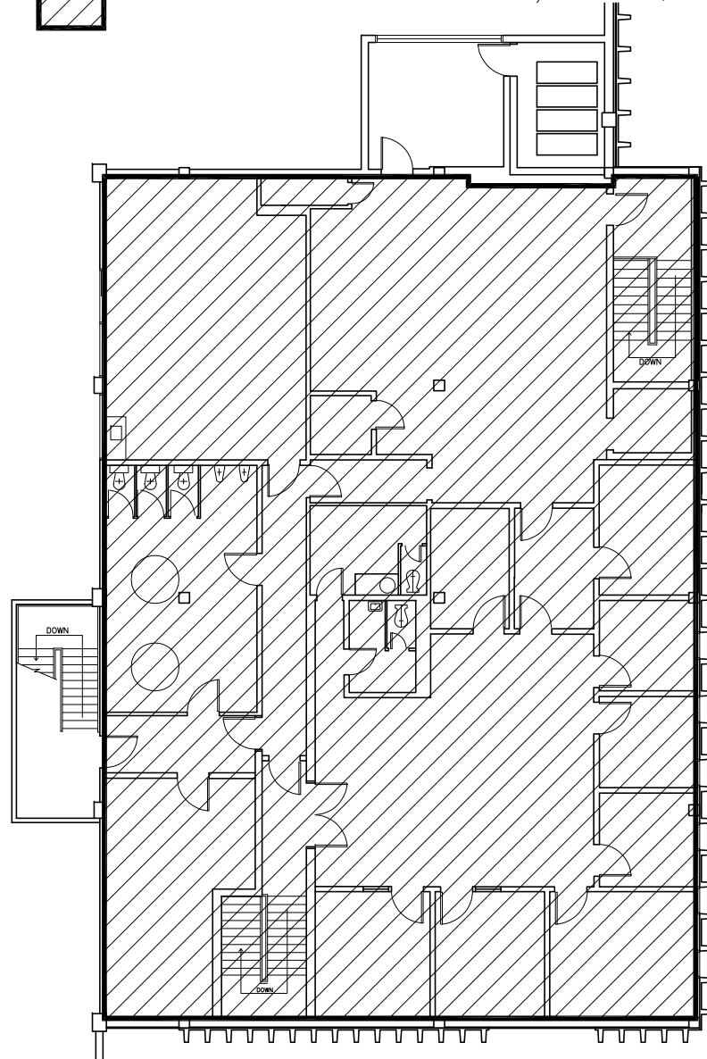
1500 PLESSIS BUILDING "B" SECOND FLOOR PLAN
