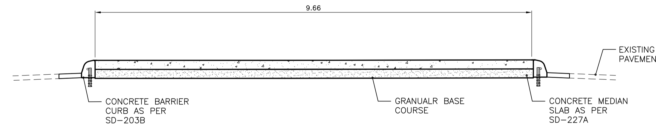
A ELGIN AVENUE WEST & KEEWATIN STREET SECTION 1:50H 1:25V
