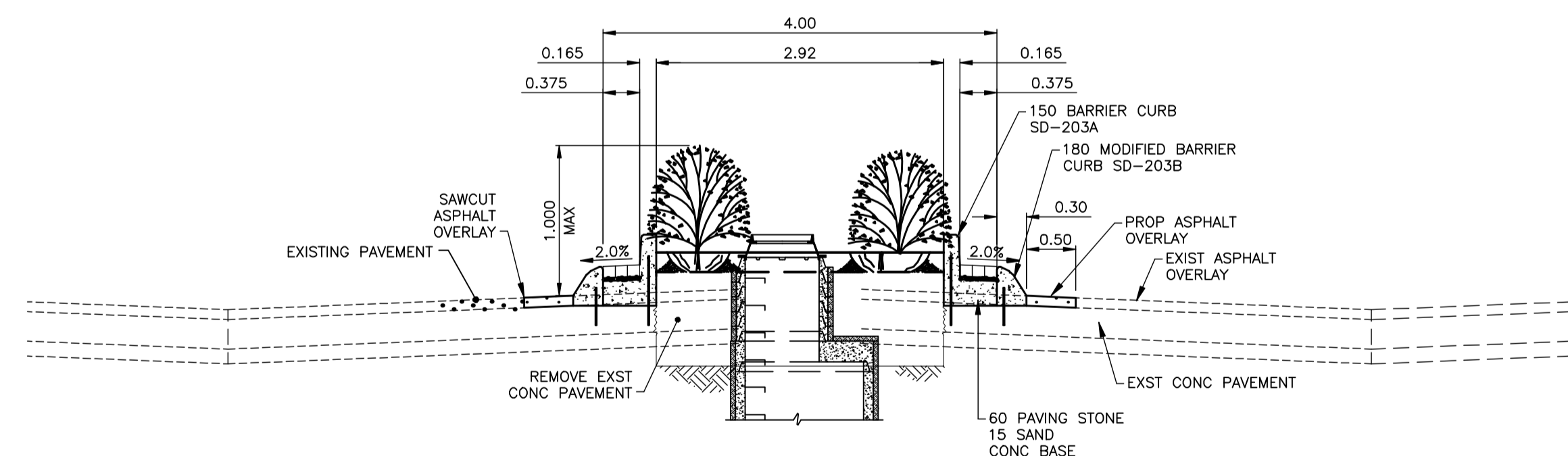
A ELGIN AVENUE WEST & ODDY STREET SECTION 1:50H 1:25V
