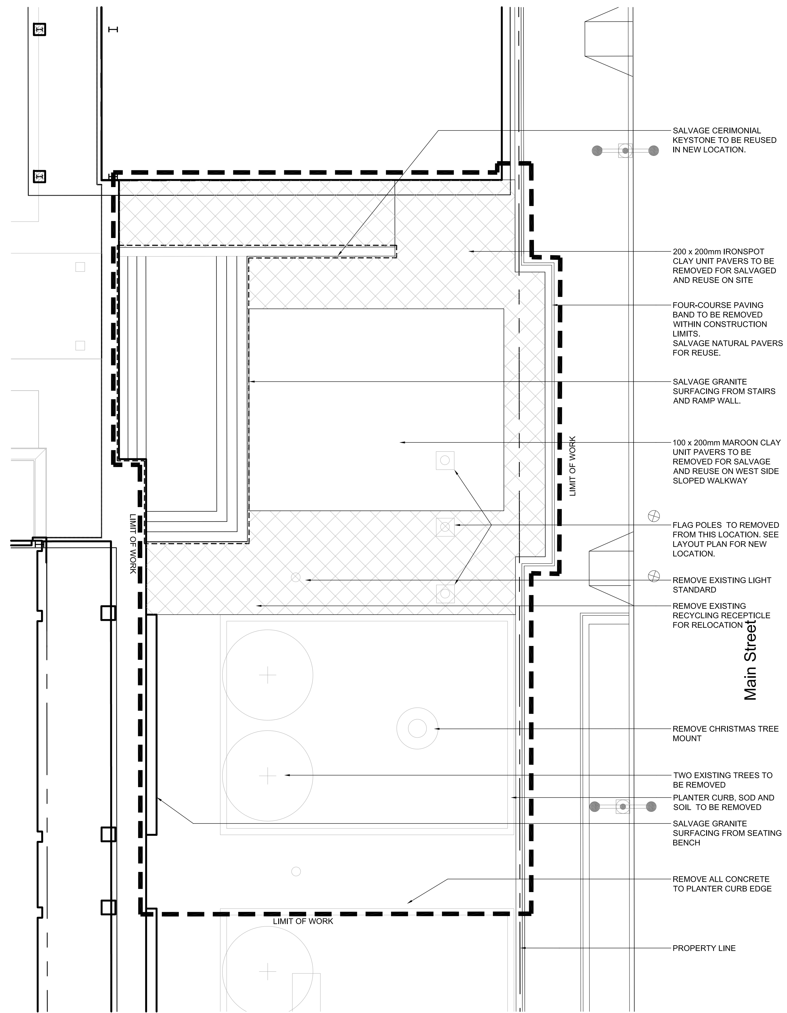
2 LAYOUT PLAN - EAST L00 1:100
