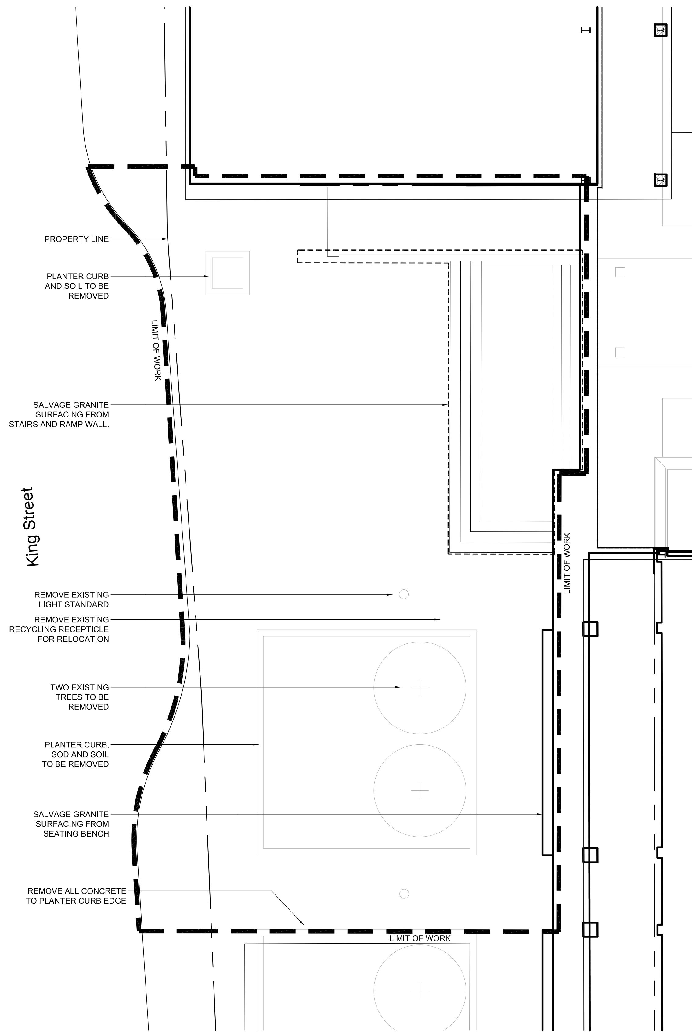
1 LAYOUT PLAN - WEST L00 1:100
