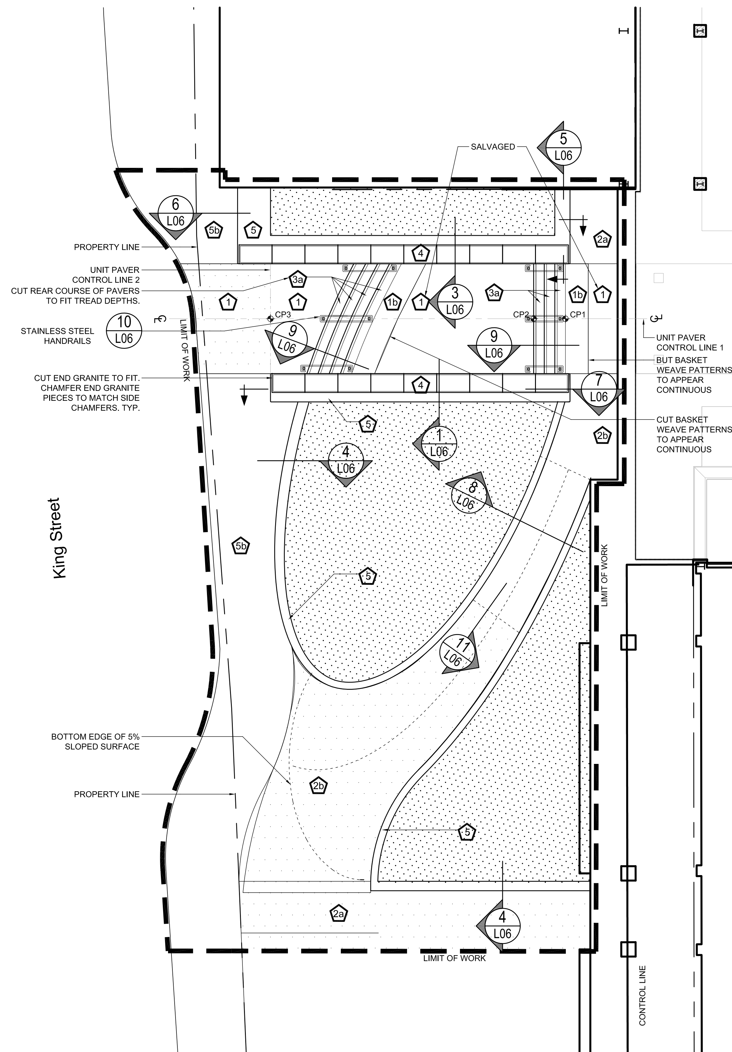
1 L03 LAYOUT PLAN - WEST 1:100
