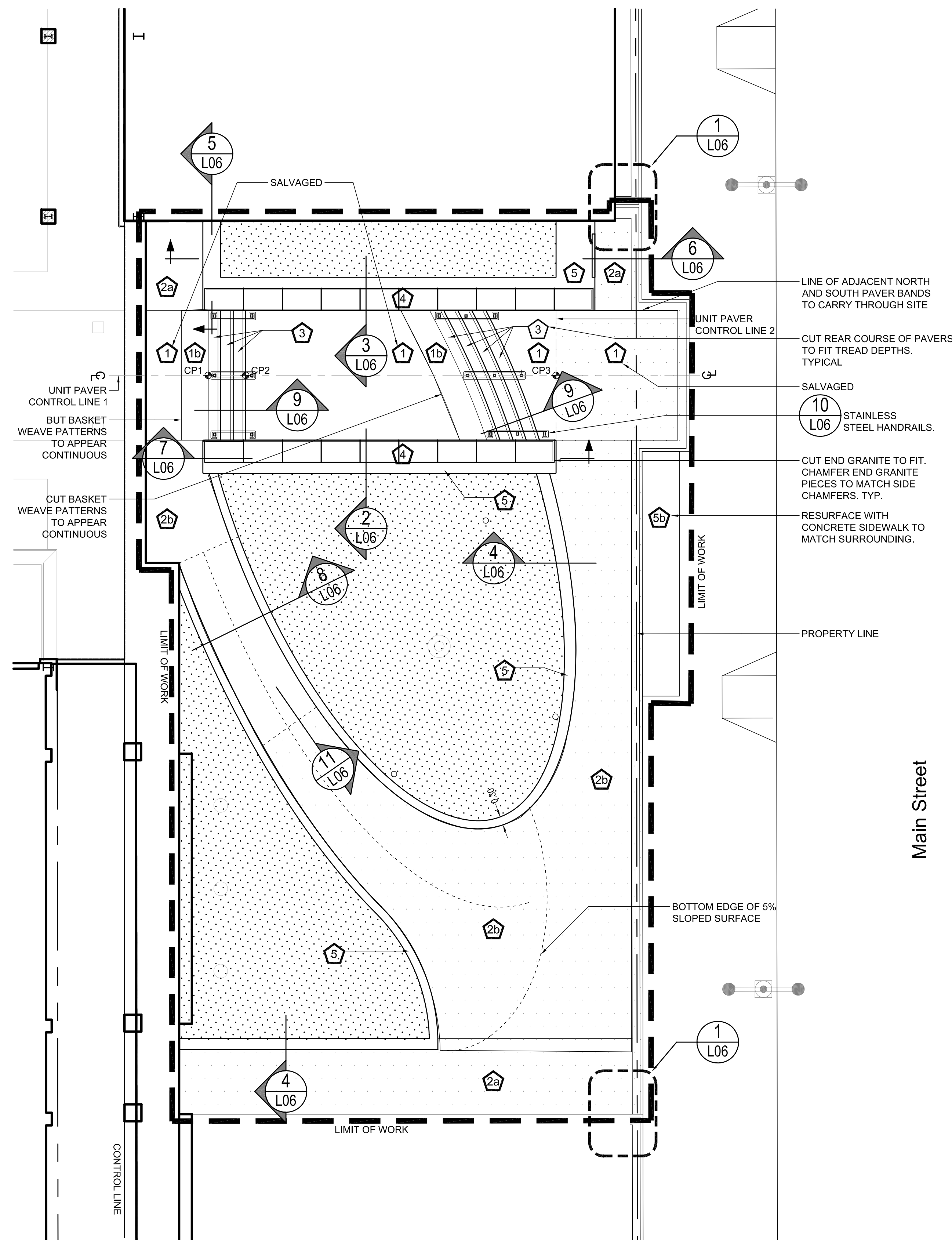
2 L03 LAYOUT PLAN - EAST 1:100
