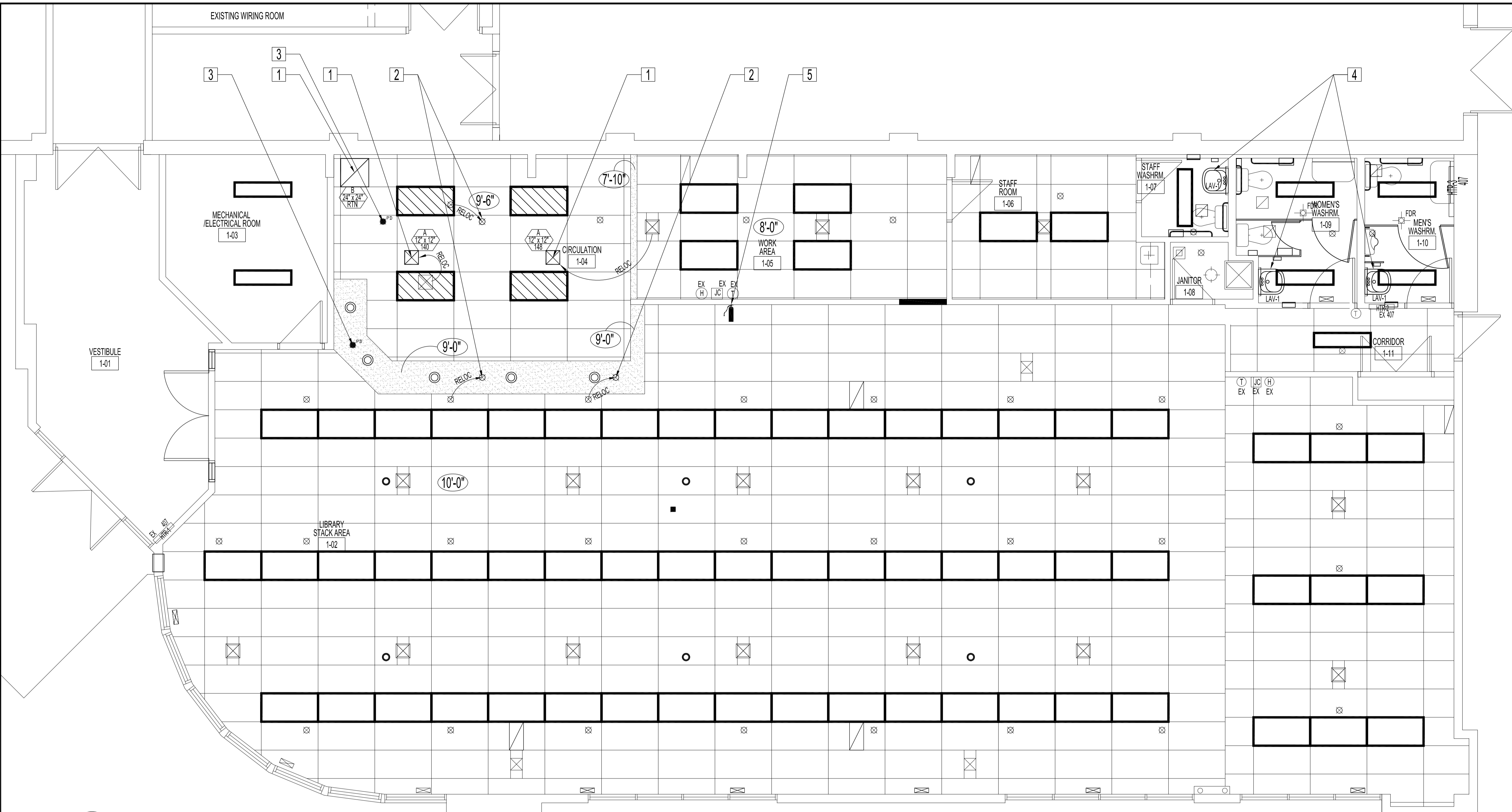
REFLECTED MAIN FLOOR PLAN - REFLECTED CEILING MECHANICAL & PLUMBING RENOVATION DOORS, FIXTURES & CONTROLS SHOWN FOR CLARITY SCALE: 1/4"=1'-0"
