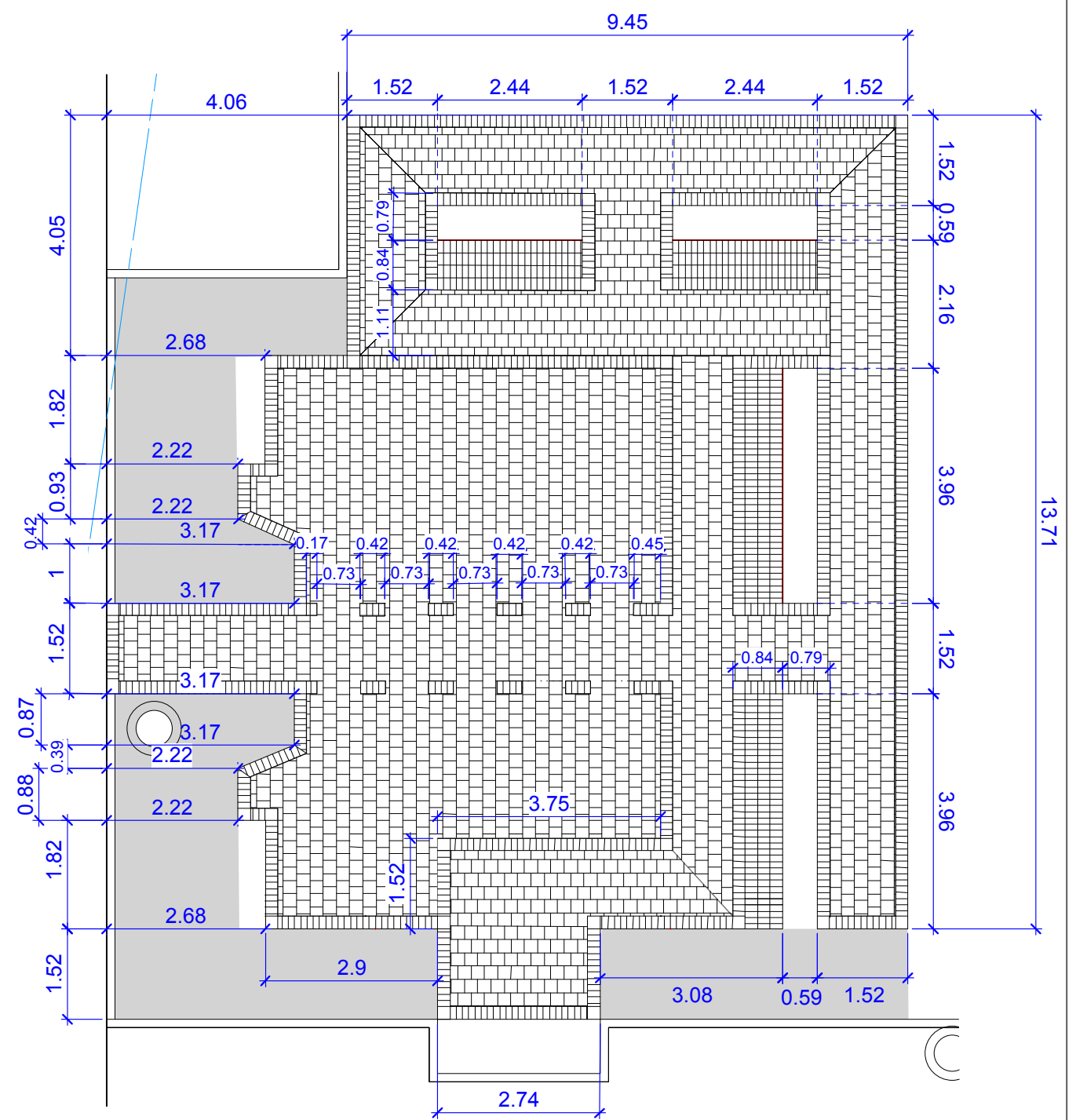
PAVING LAYOUT Scale - 1:100
