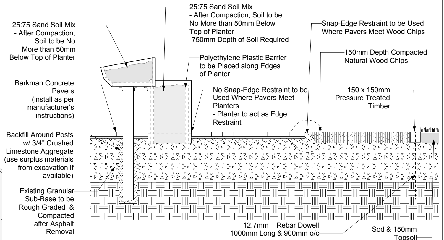
ACCESSIBLE PLANTER DETAIL Scale - 1:50
