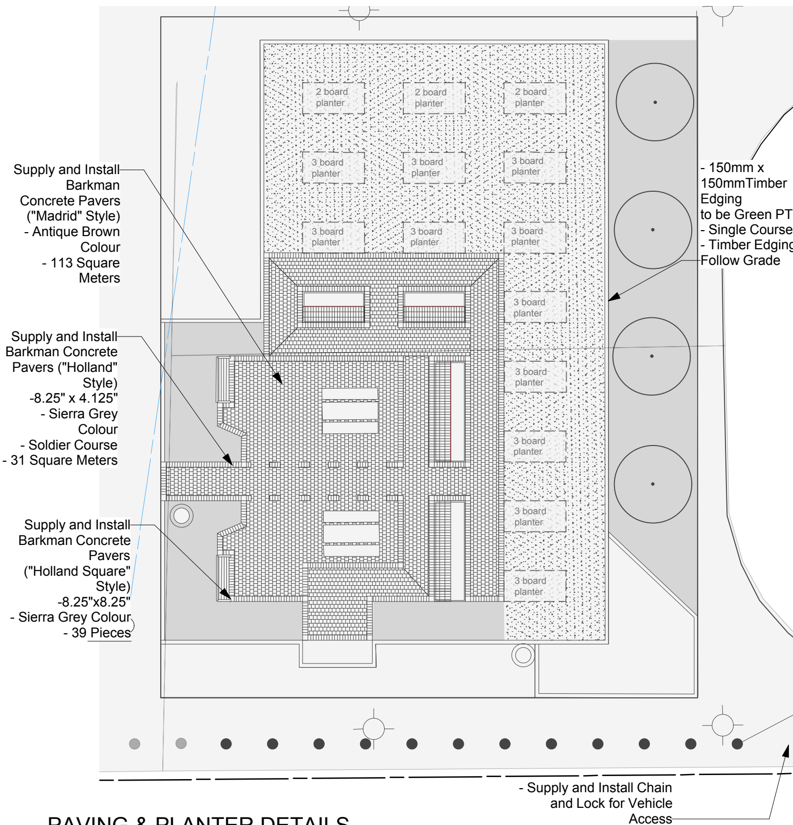
PAVING & PLANTER DETAILS Scale - 1:150
