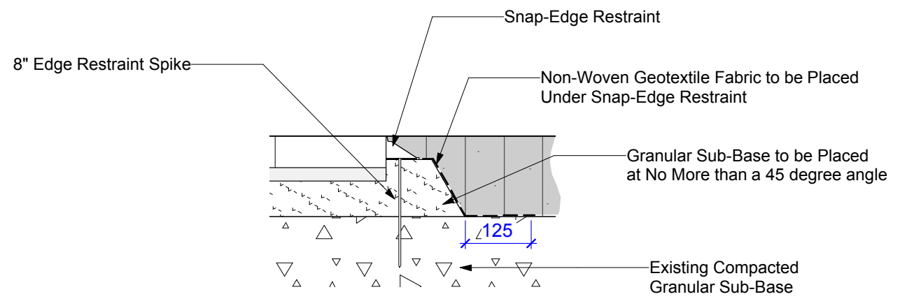
SNAP EDGE DETAIL Scale - 1:10
