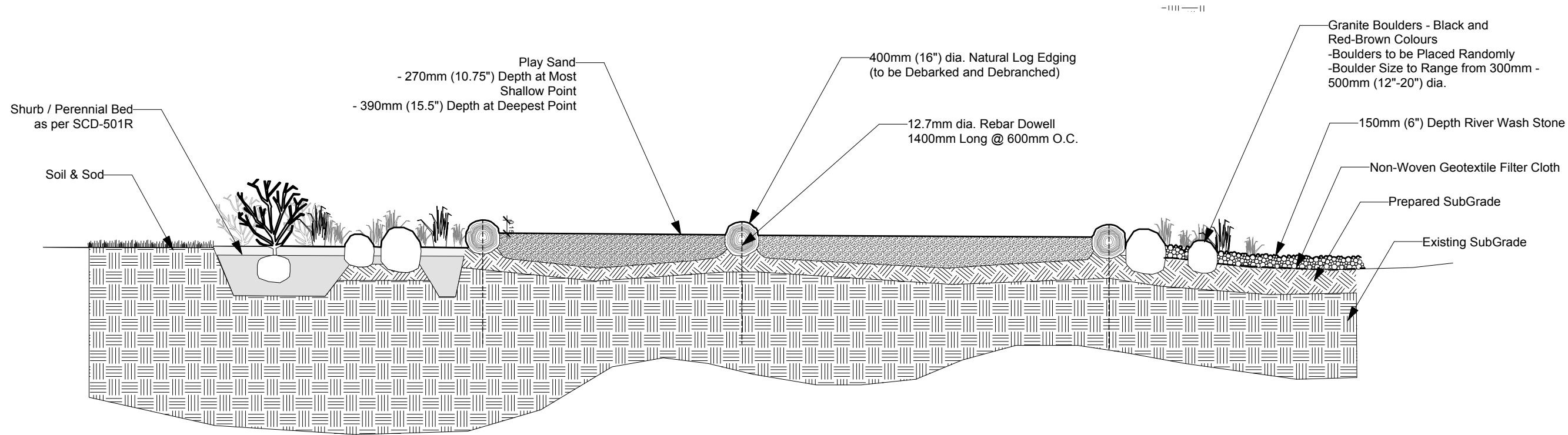
Site Section 'C' - Sand Play Area SCALE - 1:50
