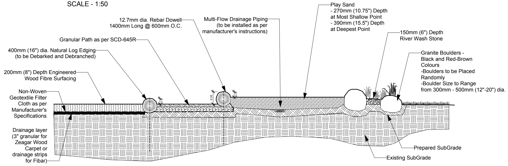
Site Section 'D' - Sand Play Area SCALE - 1:50
