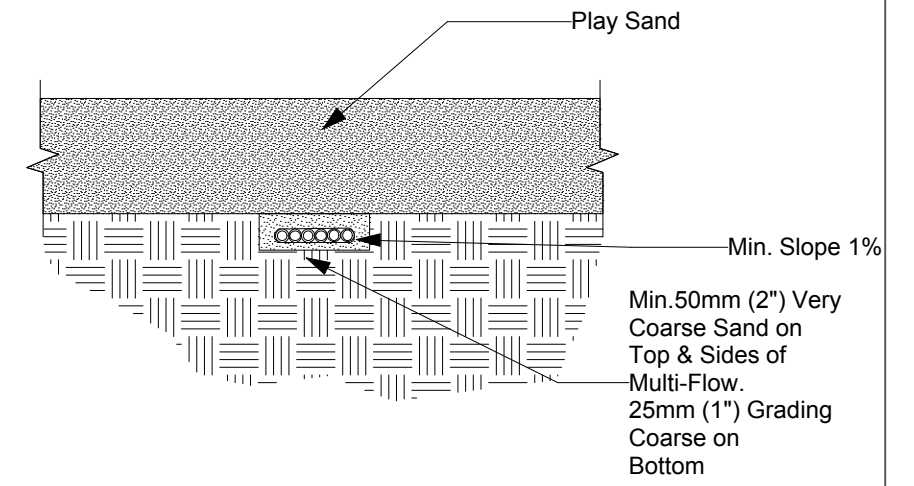
Subsurface Drainage Under Sand Play SCALE - 1:25
