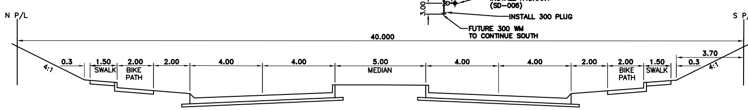
TYPICAL CROSS SECTION BISON DRIVE SCALE: HOR. 1:100 VER. 1:50
