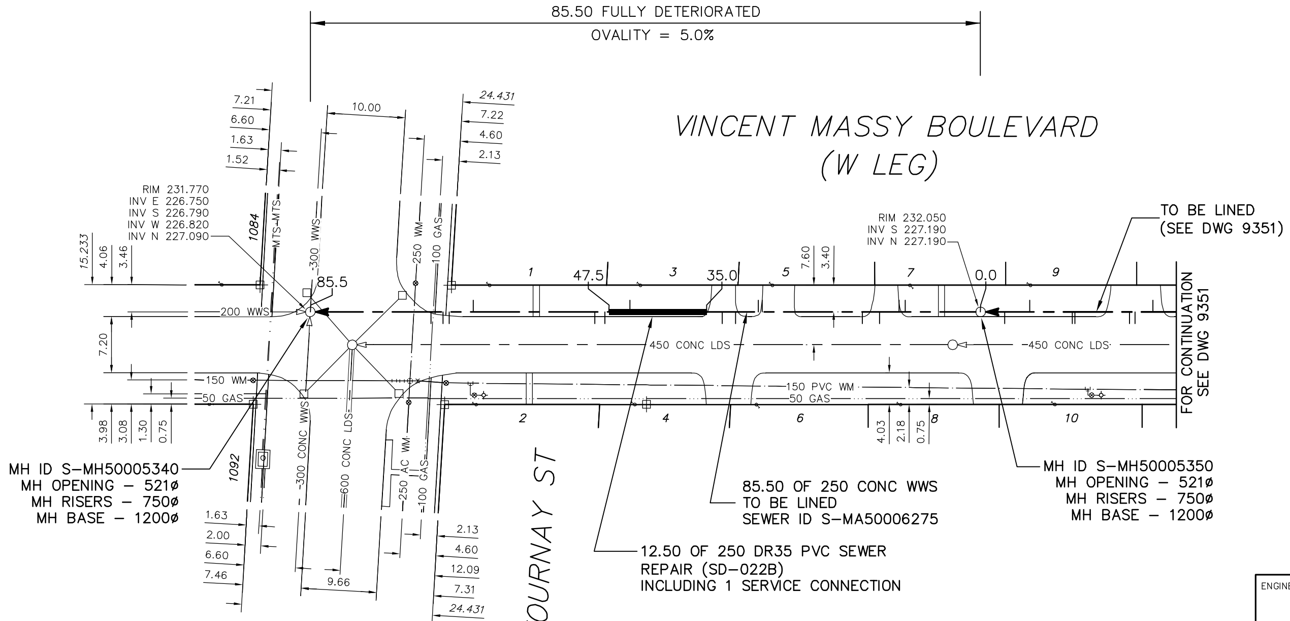
SEWER JUNCTION INFORMATION FROM SEWER VIDEO INSPECTION SEWER ID S-MA50006275
