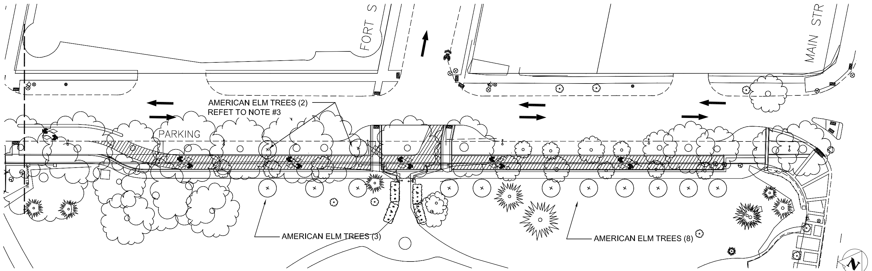
1 TREE PLANTING GARRY TO MAIN L103 SCALE 1:500
