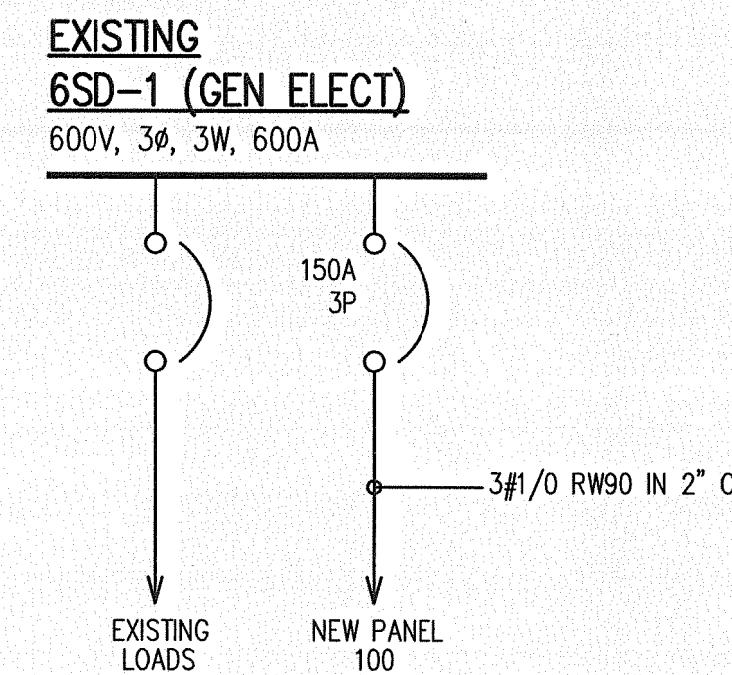
3 SINGLE LINE E1.0 SCALE: NTS
