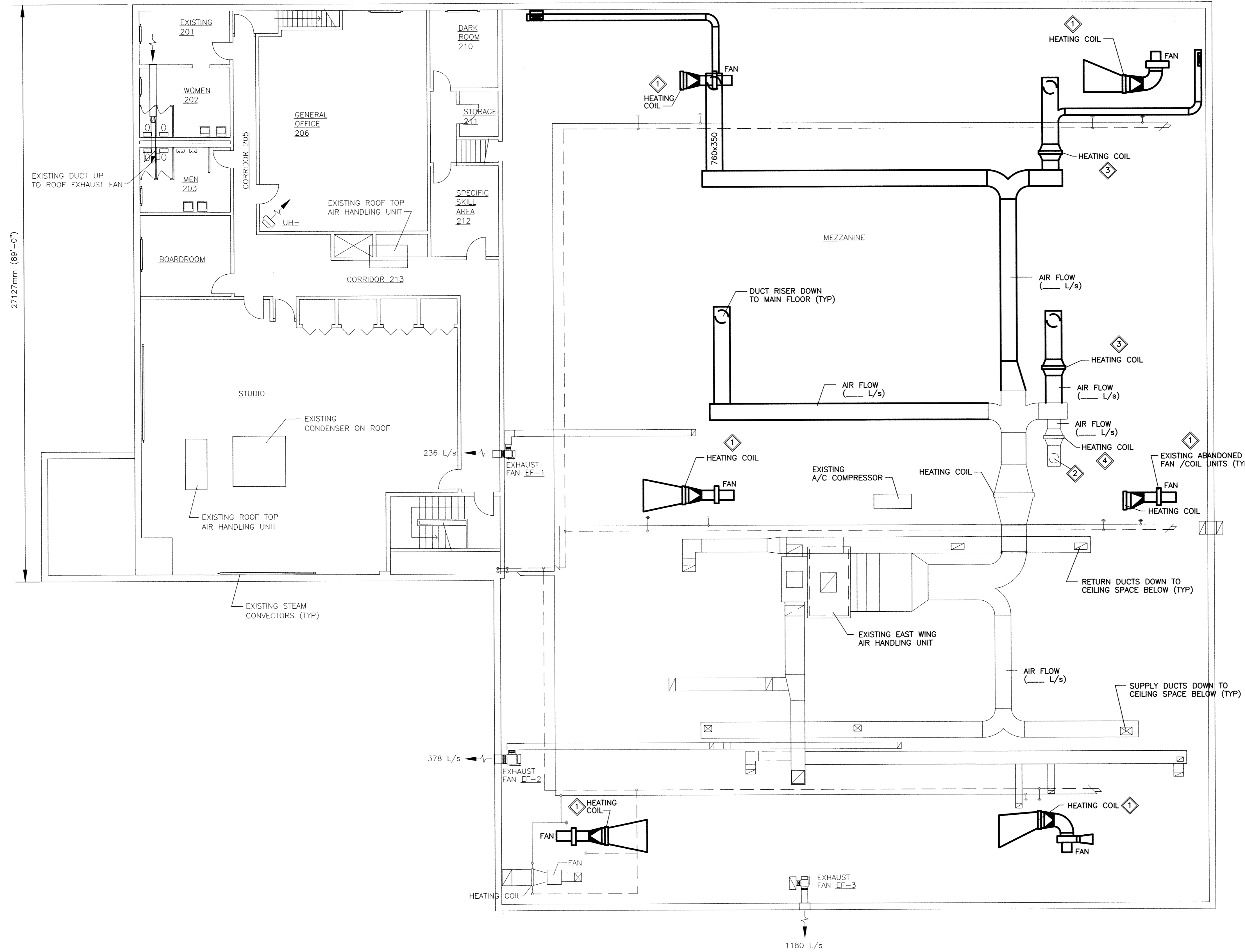
1 MEZZANINE/SECOND FLOOR PLAN – DEMOLITION
