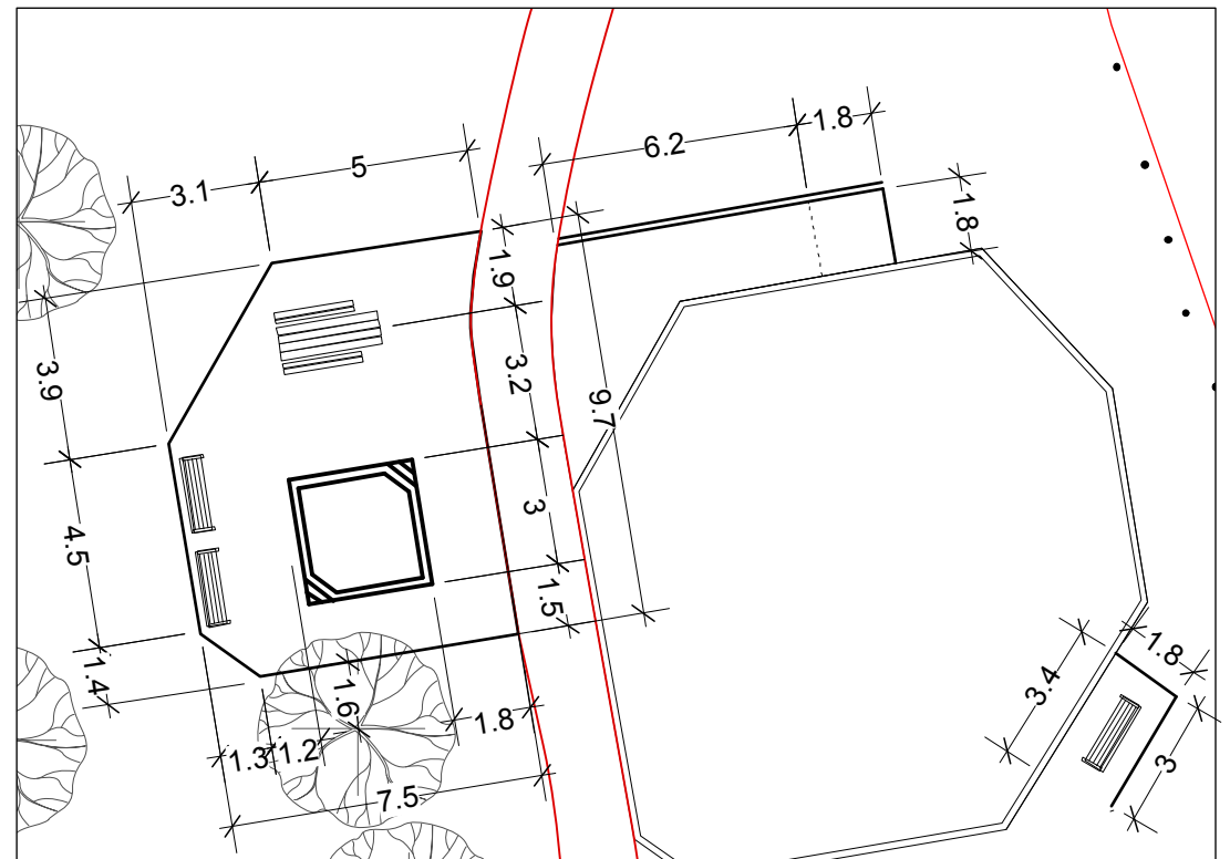
LAYOUT OF SAND BOX, RAMP AND GRANULAR SITTING AREA 1:200
