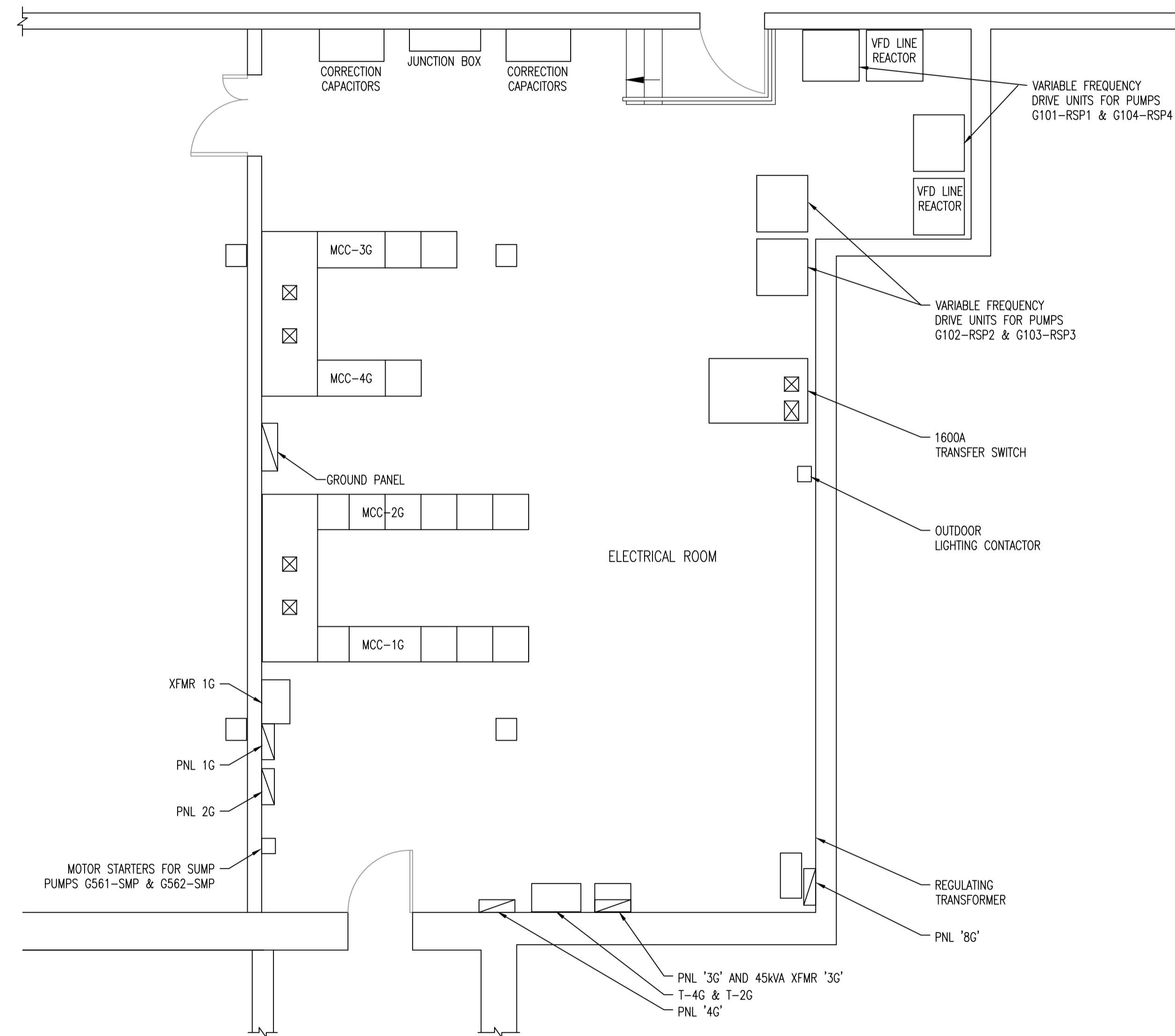
GRIT AREA ELECTRICAL ROOM 1:50
