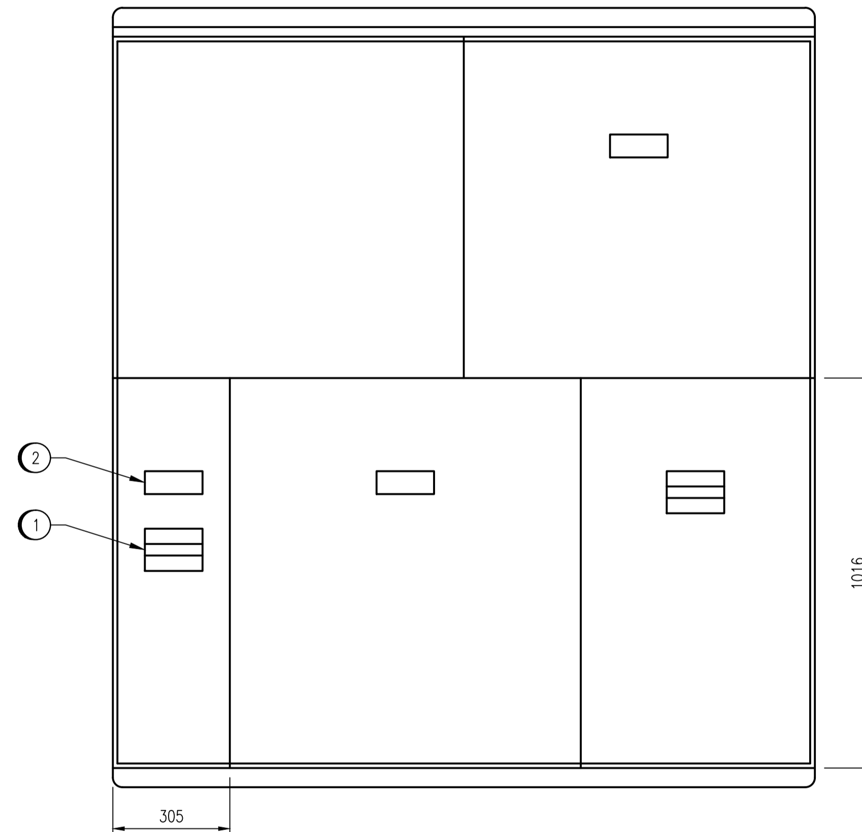
FRONT ELEVATION LESS OUTER DOOR SCALE: 1 : 10
