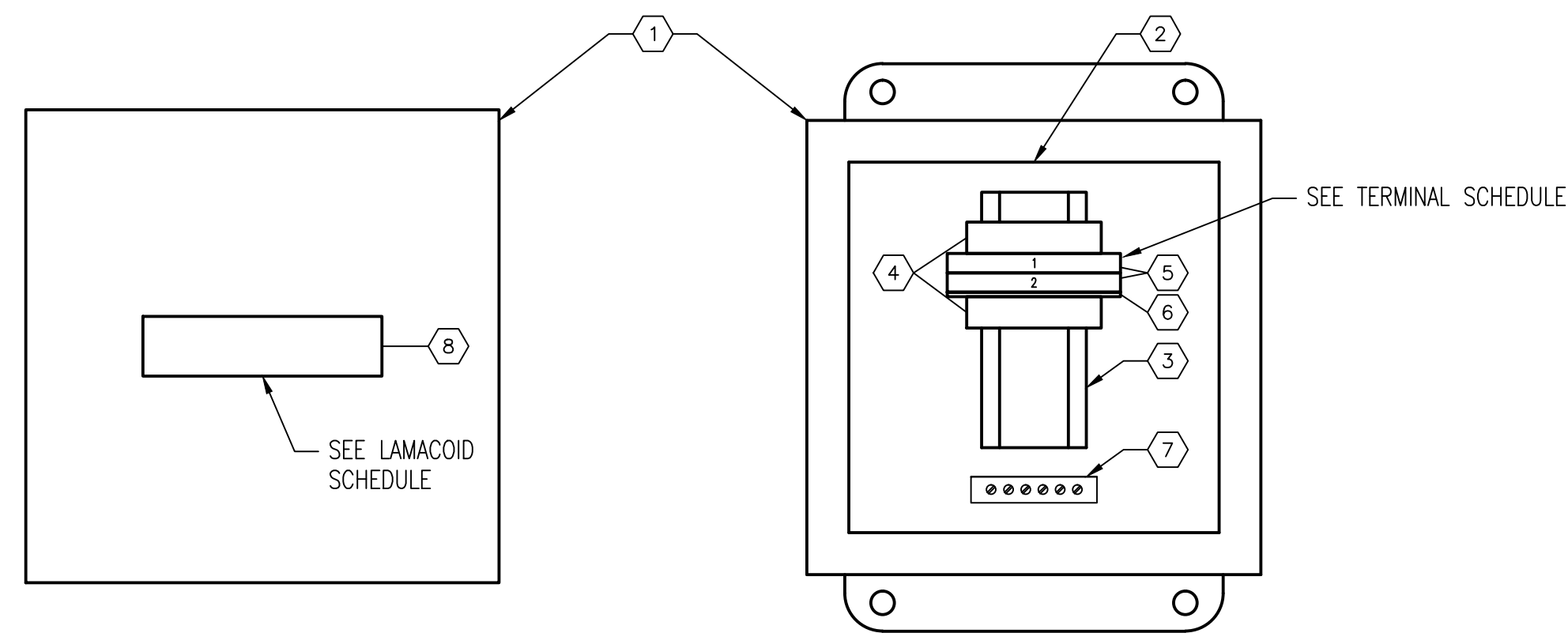
EXTERIOR PANEL VIEW SCALE: 1 : 2
