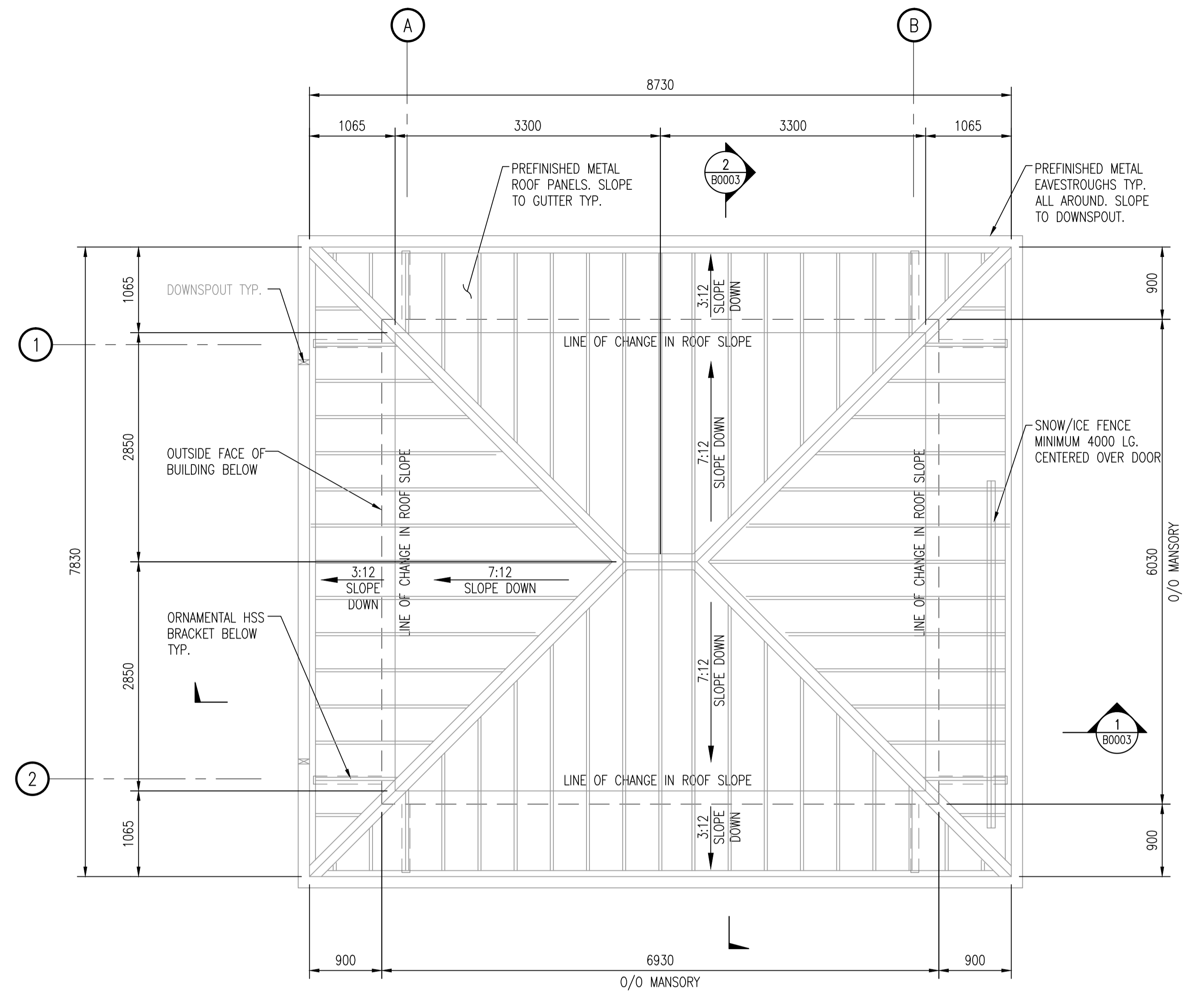
ROOF PLAN SCALE: 1 : 40
