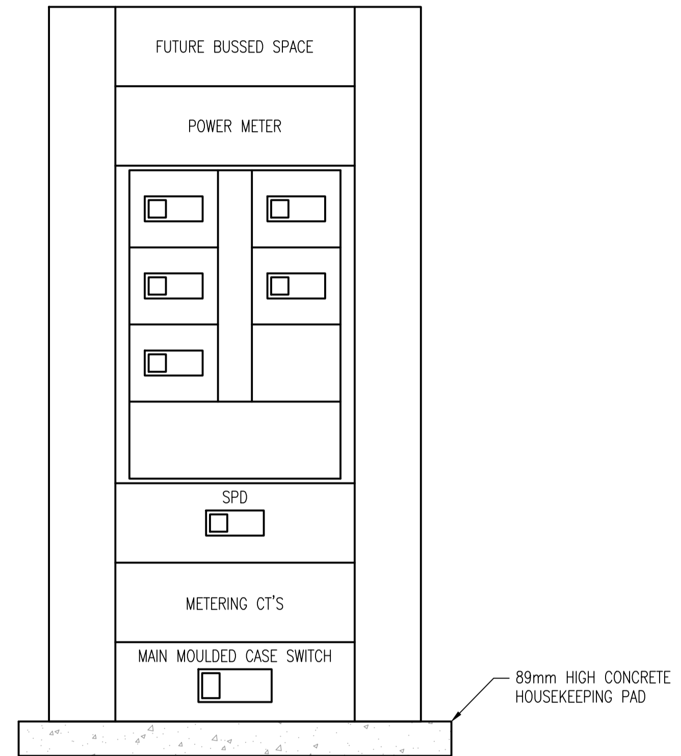
MAIN DISTRIBUTION PANEL ELEVATION SCALE: NTS
