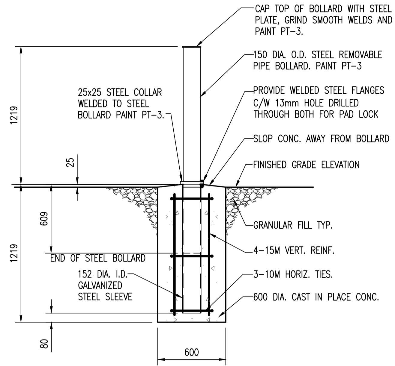
REMOVABLE BOLLARD DETAIL SCALE: 1 : 20
