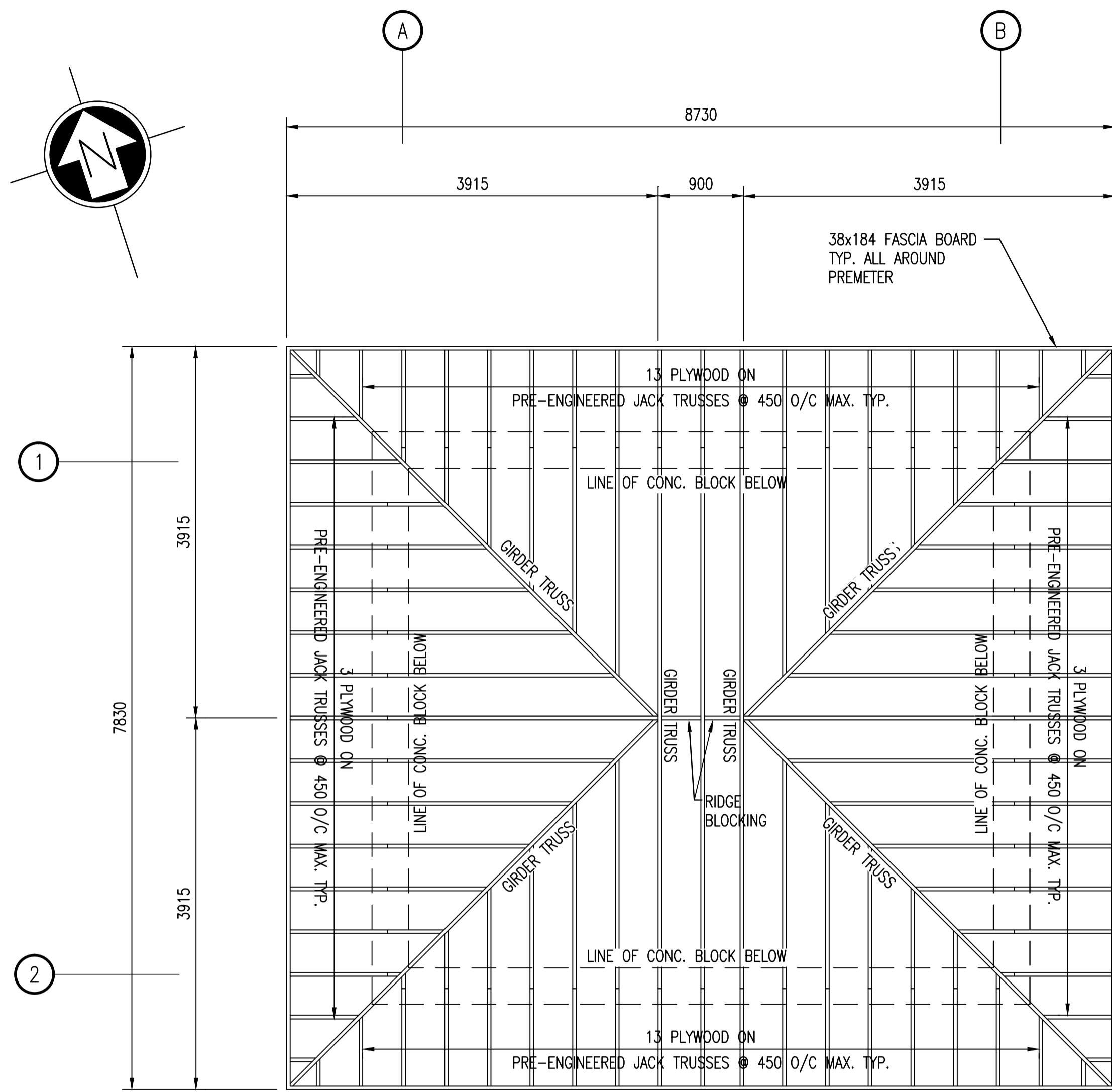
ROOF FRAMING PLAN SCALE: 1 : 40
