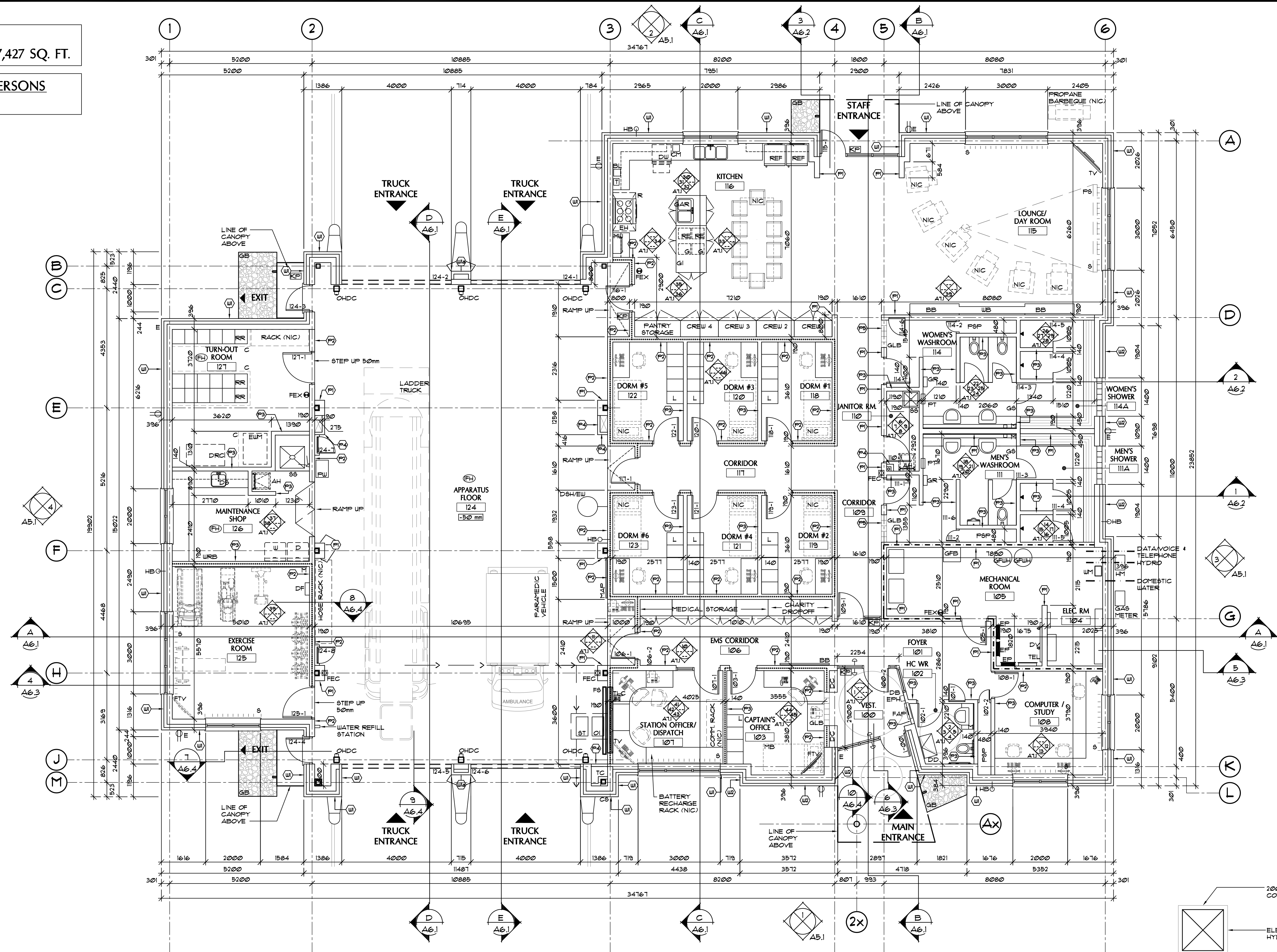
1 FLOOR PLAN SCALE 1: 1/8
