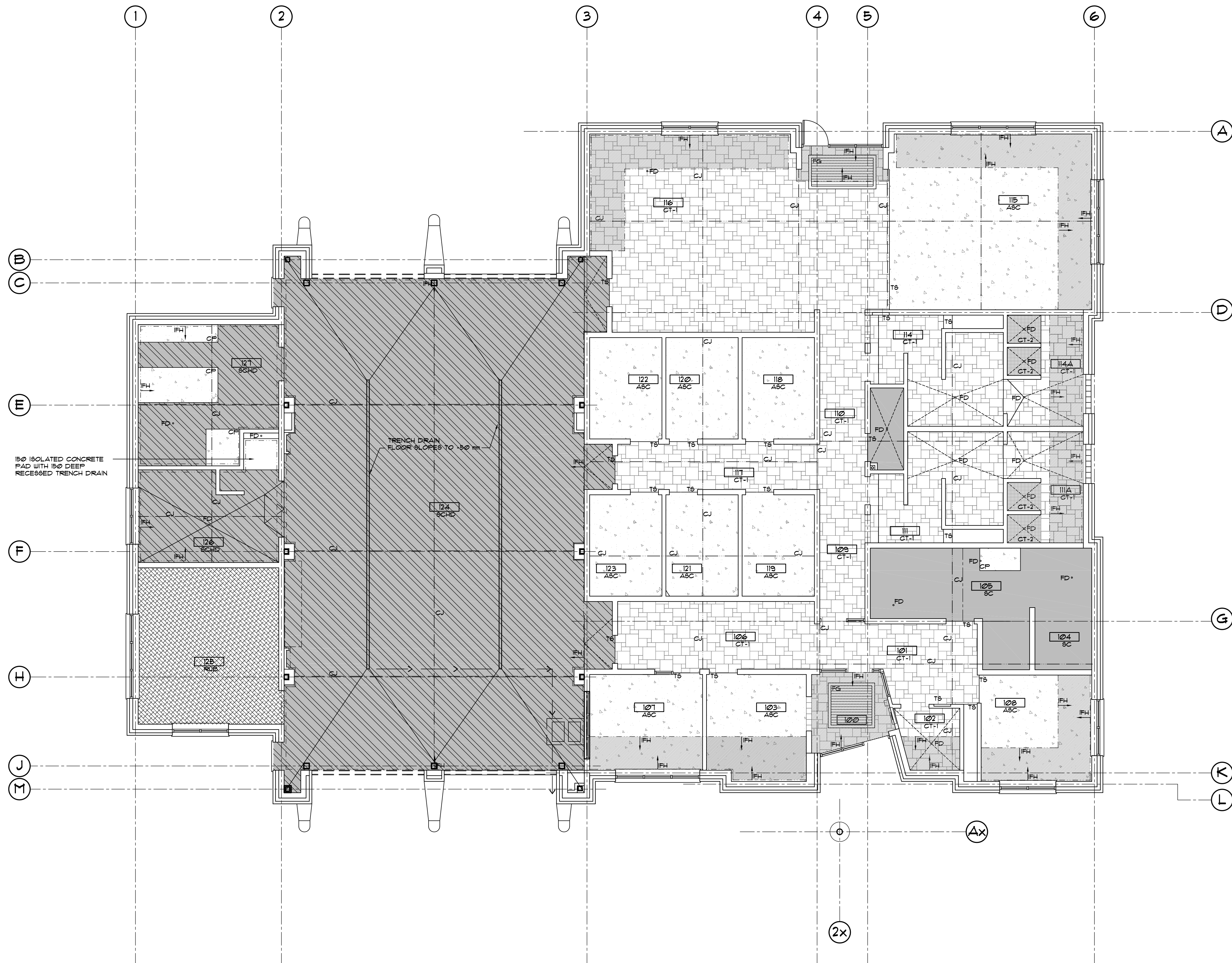
1 A2.2 FLOOR FINISH PLAN SCALE 1:75
