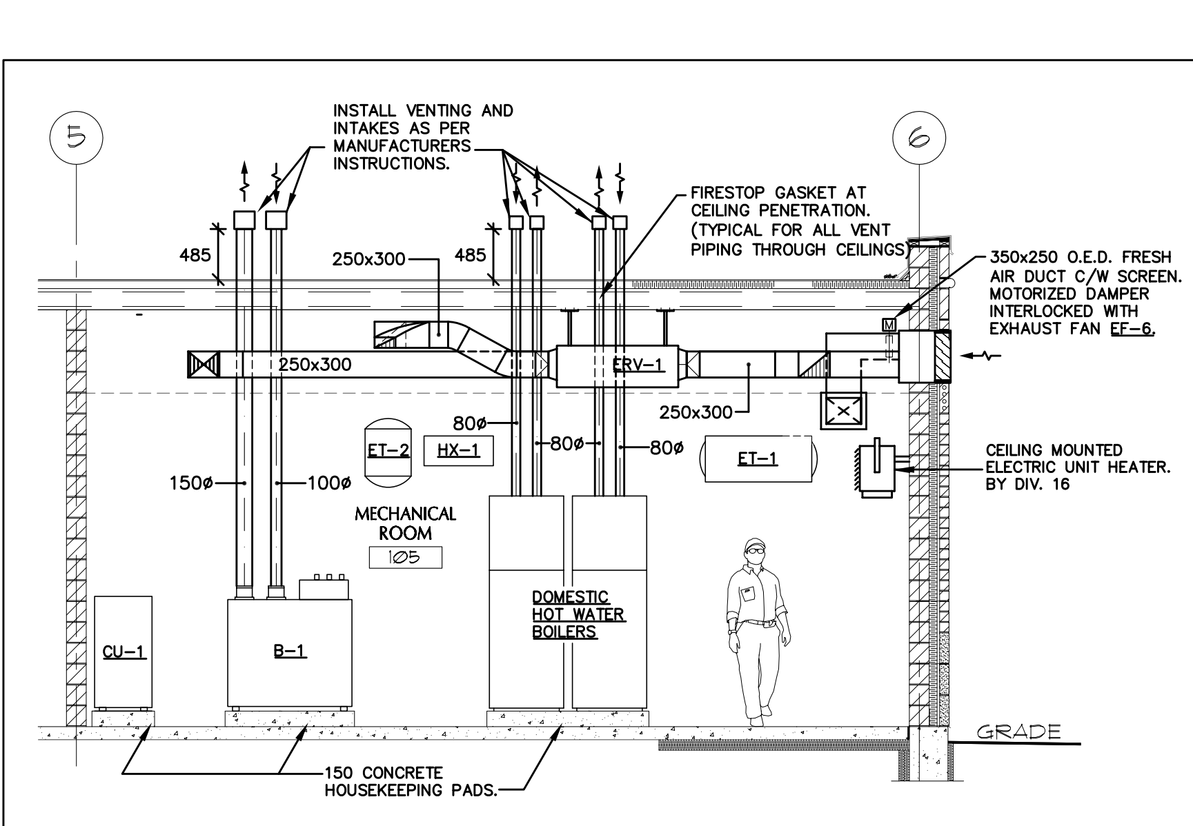
A M4.1 SECTION - MECHANICAL ROOM SCALE 1: 50
