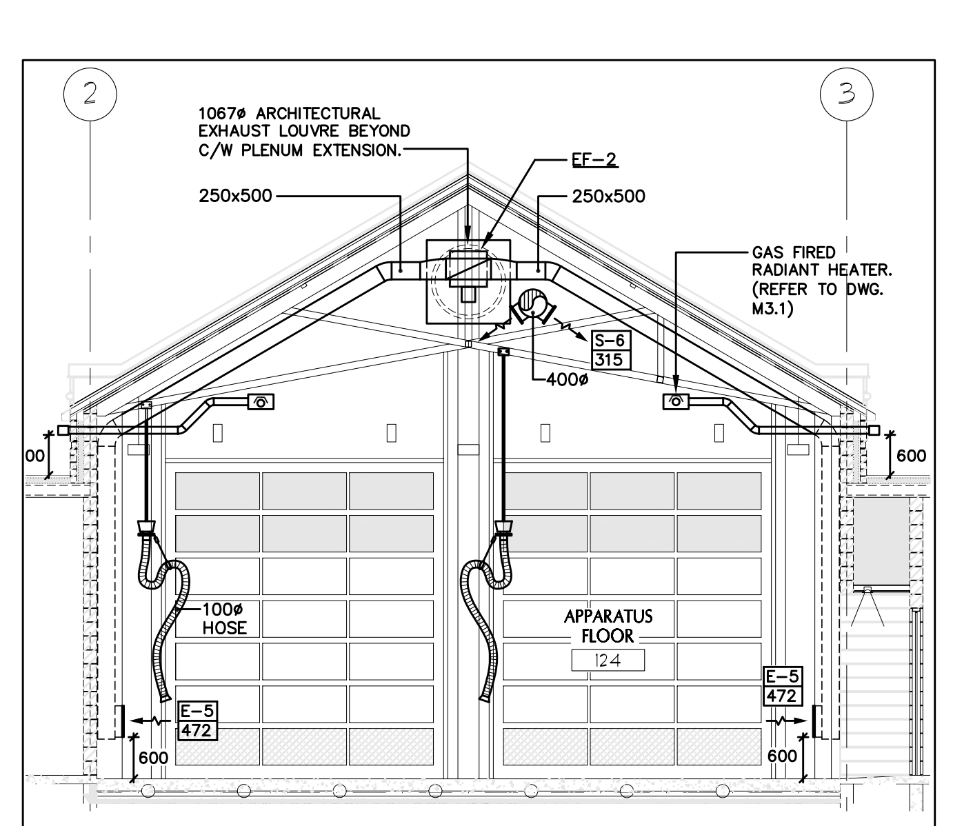
B M4.1 SECTION VIEW - APPARATUS FLOOR SCALE 1: 15
