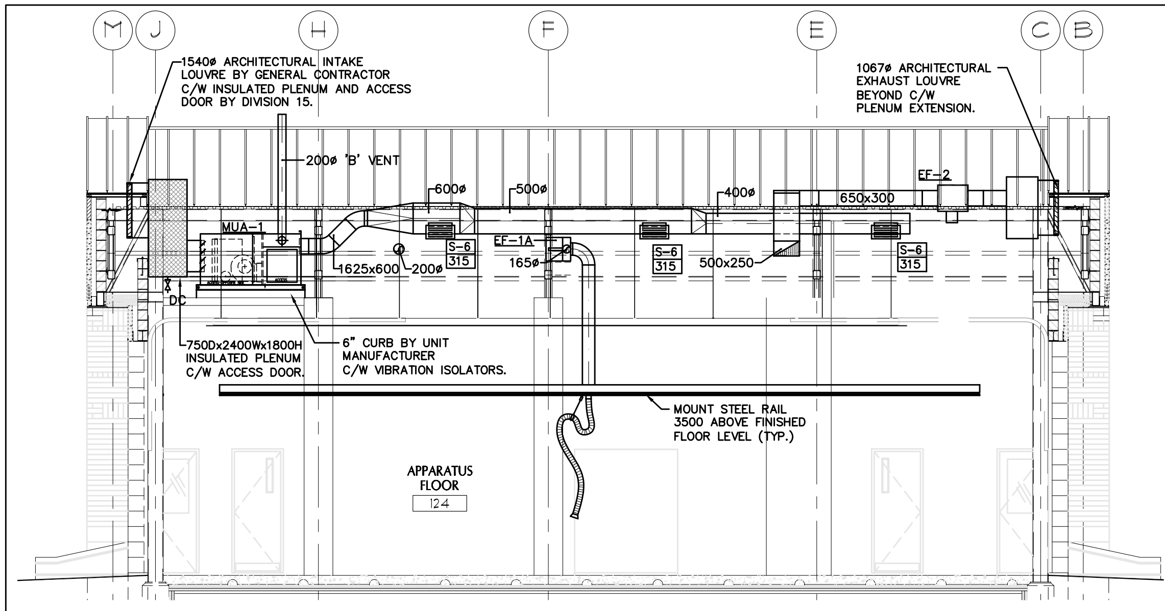
C M4.1 SECTION VIEW - APPARATUS FLOOR SCALE 1: 15
